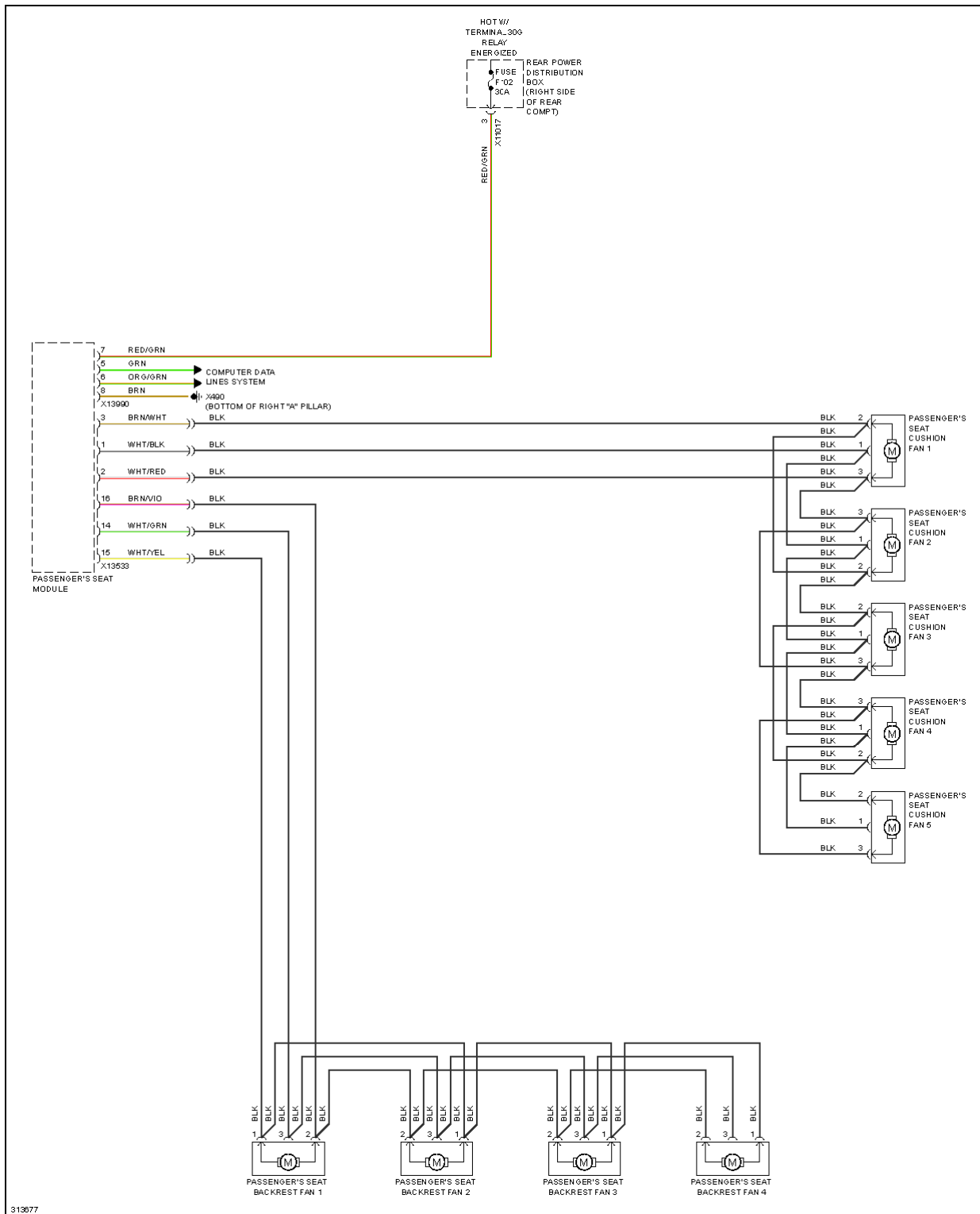
Fig. 100: Seat Ventilation Circuit (2 of 2)
