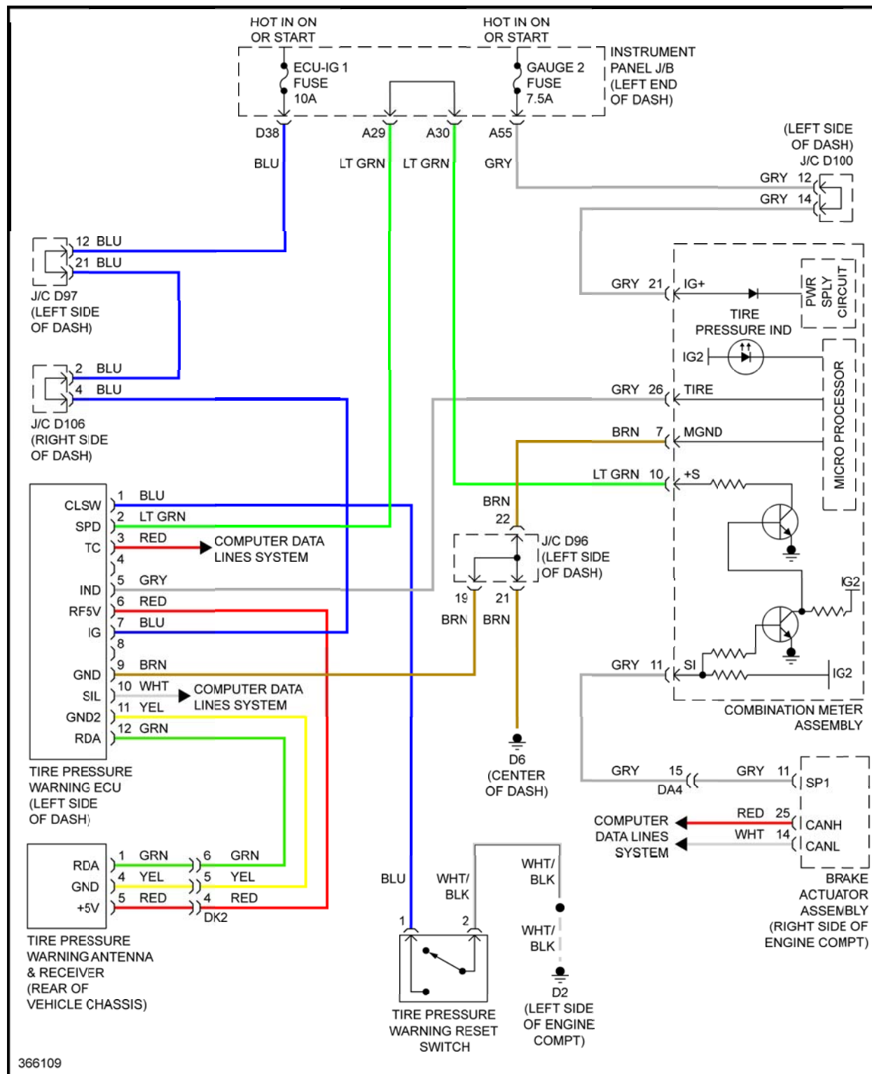
Fig. 125: Tire Pressure Monitoring Circuit
