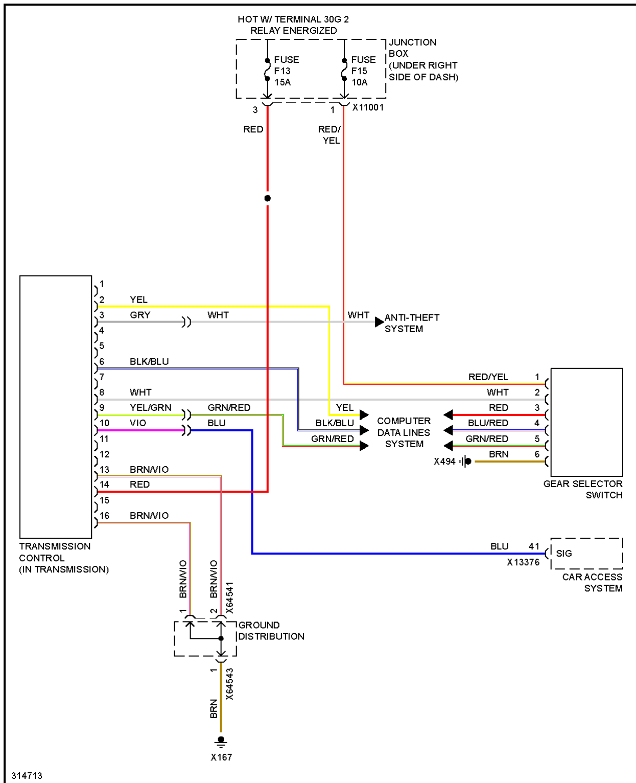
Fig. 125: 3.0L Twin Turbo, A/T Circuit
