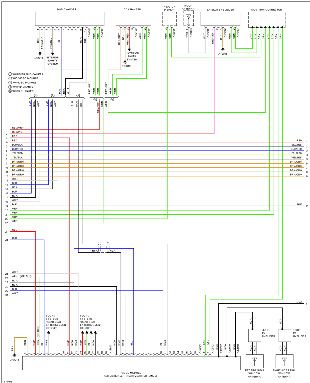
Fig. 113: Radio Circuit, W/O CIC & W/ HIFI Radio (2 of 3)
