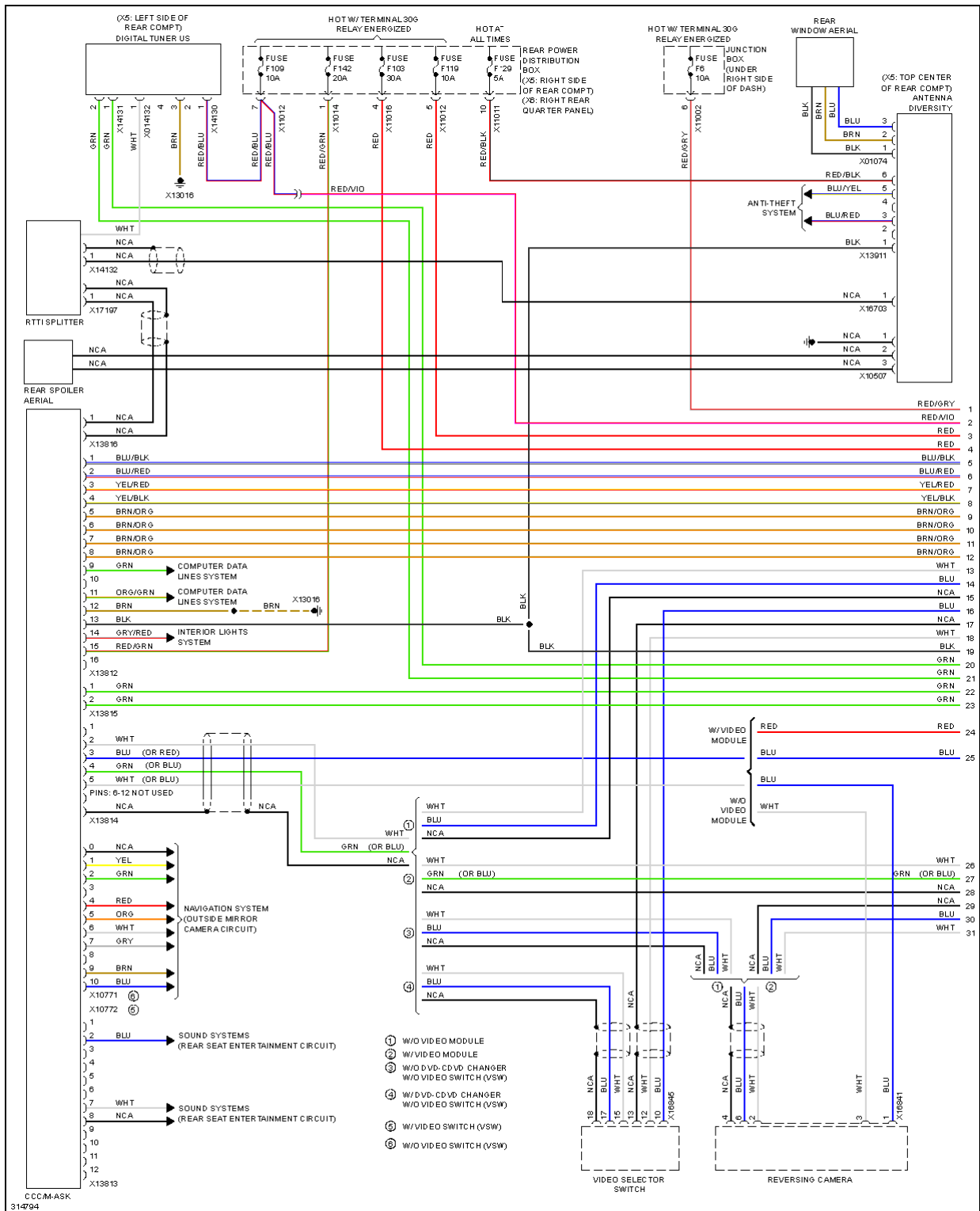
Fig. 112: Radio Circuit, W/O CIC & W/ HIFI Radio (1 of 3)
