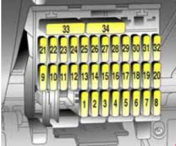
Vauxhall Omega B – fuse box diagram
