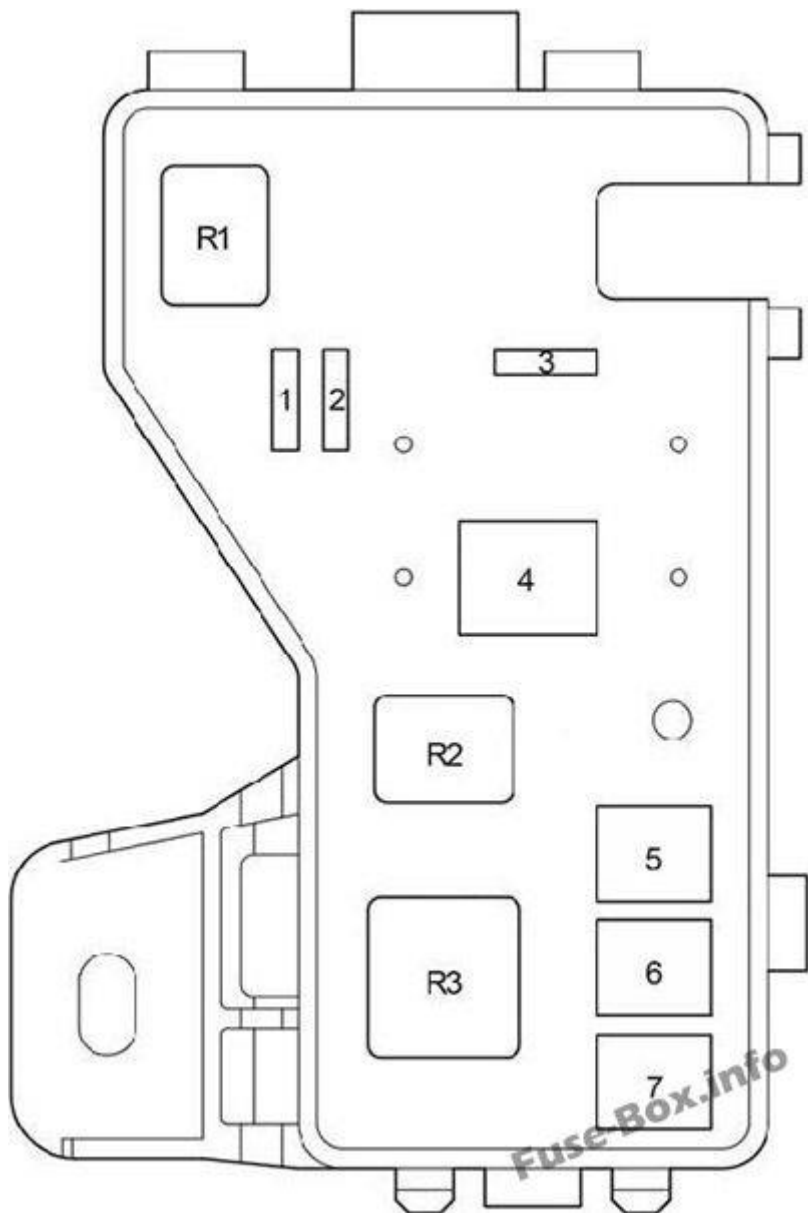
Engine Compartment Additional Fuse Box (1ZZ-FE, 3ZZ-FE)
