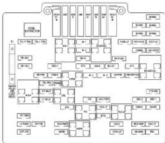
GMC Sierra mk1 – fuse box – engine
