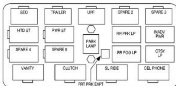
GMC Sierra mk1 – fuse box – center instrument
