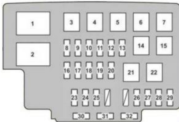
·Lexus RX 350 – fuse box diagram – engine
