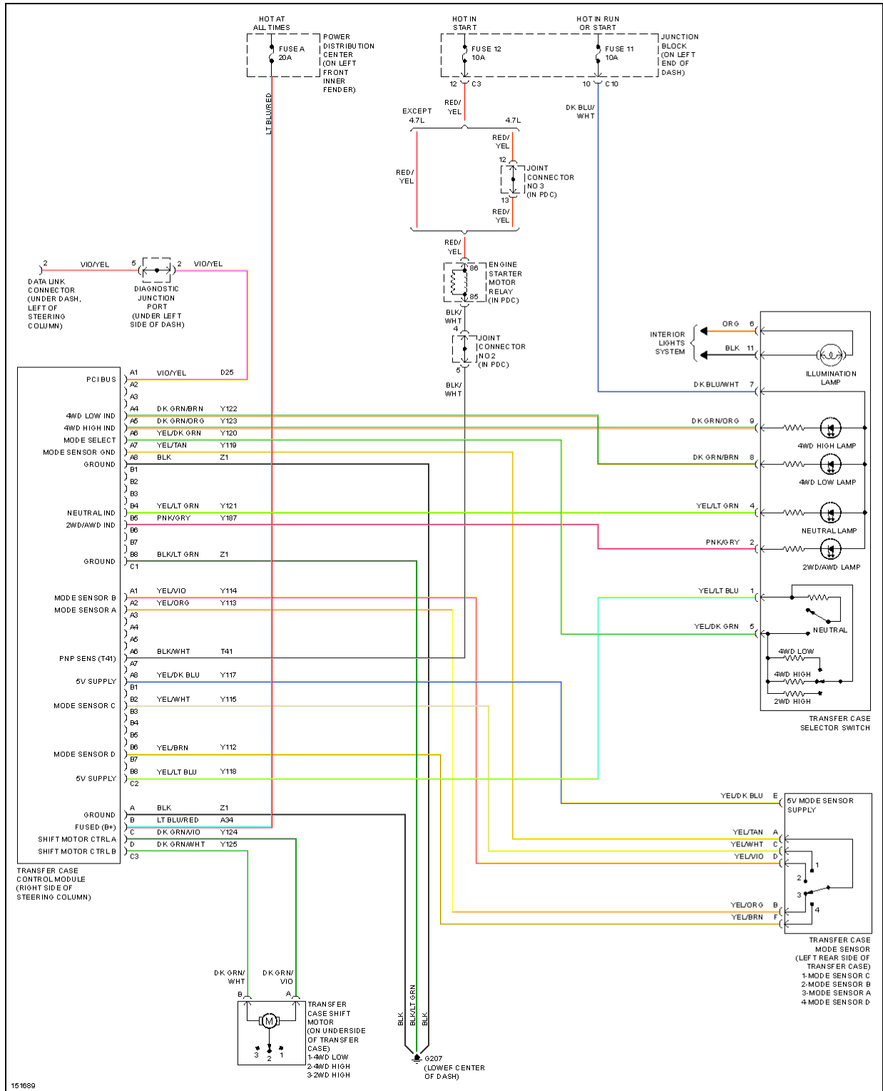
Fig. 44: Transfer Case Circuit
