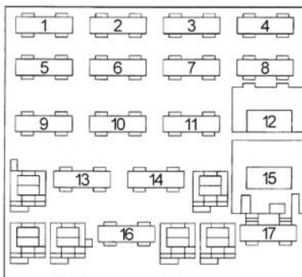
Chevrolet Celebrity – fuse box diagram
