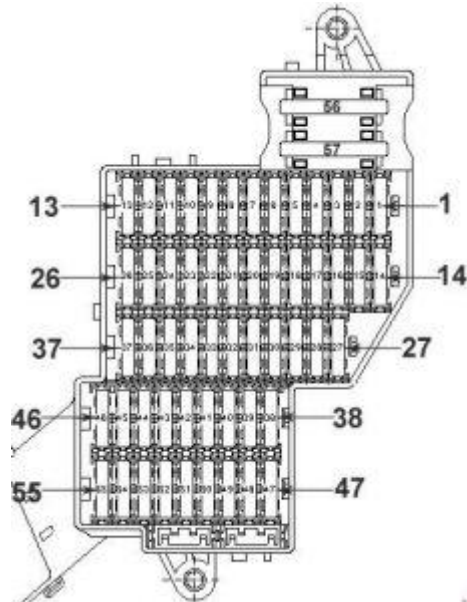
Porsche Cayenne – fuse box diagram – fuse box on
