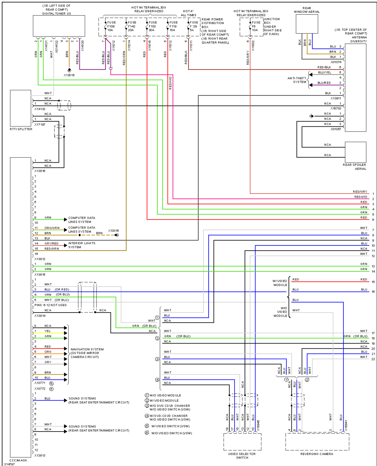
Fig. 72: Navigation Circuit, W/ Top HIFI Radio (1 of 3)
