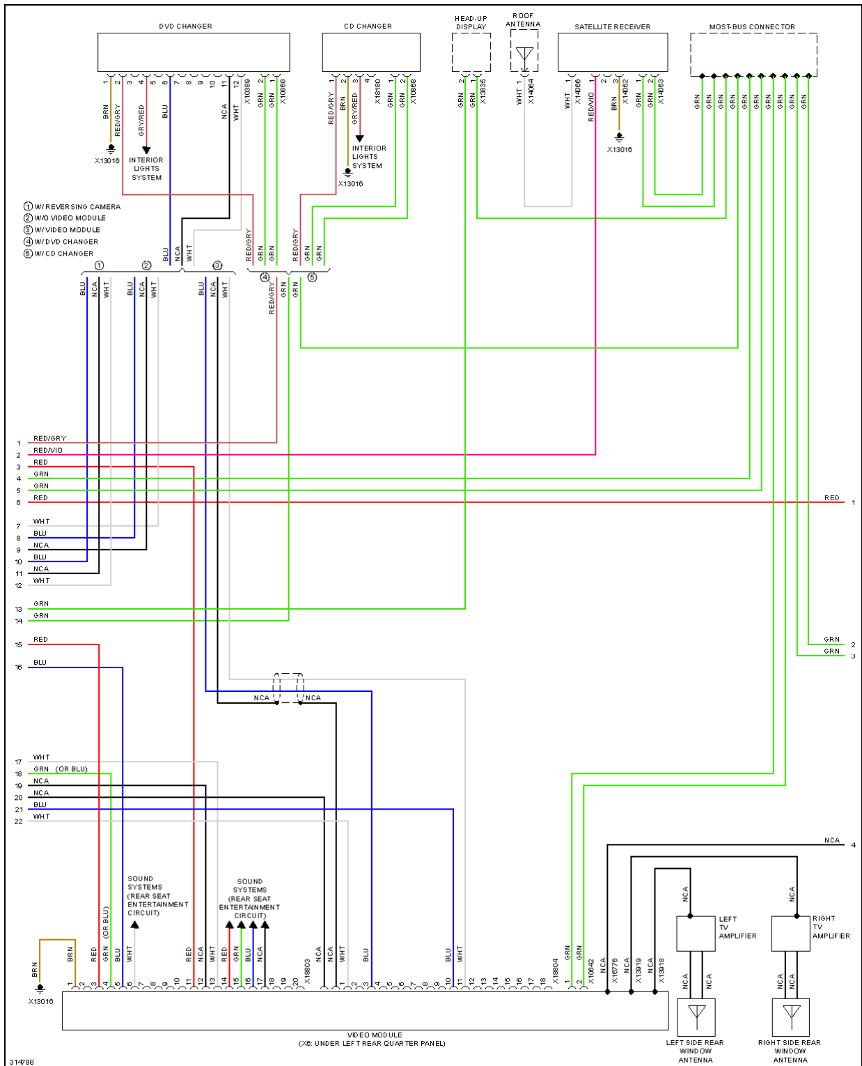
Fig. 73: Navigation Circuit, W/ Top HIFI Radio (2 of 3)
