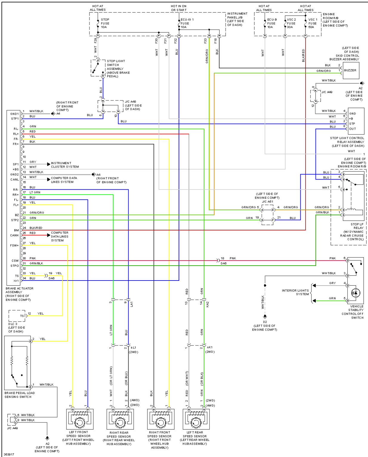
Fig. 3: Anti-lock Brakes Circuit (1 of 2)
