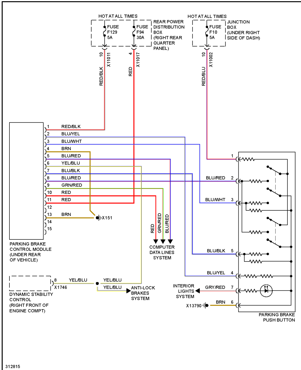
Fig. 116: Park Brake Release Circuit
