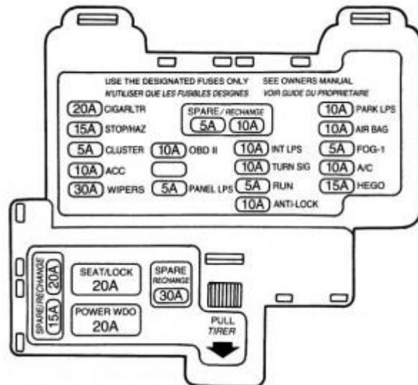
Mercury Cougar 7th Generation – fuse box – instrument panel
