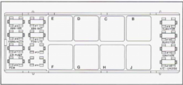
Chevrolet Camaro – fuse box – underhood
