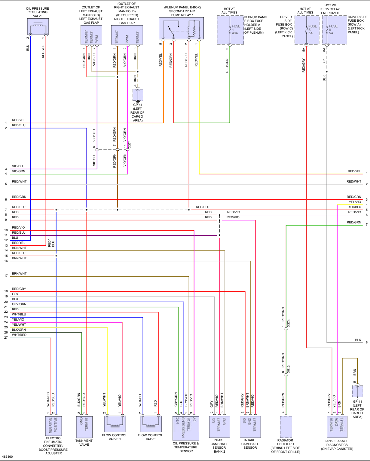
Fig 4: 3.0L Turbo, Engine Performance Circuit (4 of 6)
