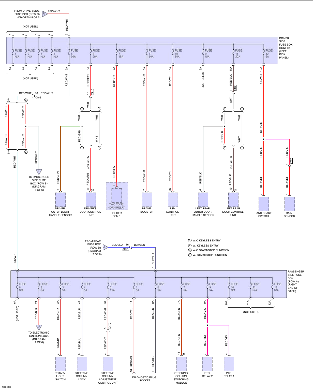
Fig 4: Power Distribution Circuit (4 of 6)
