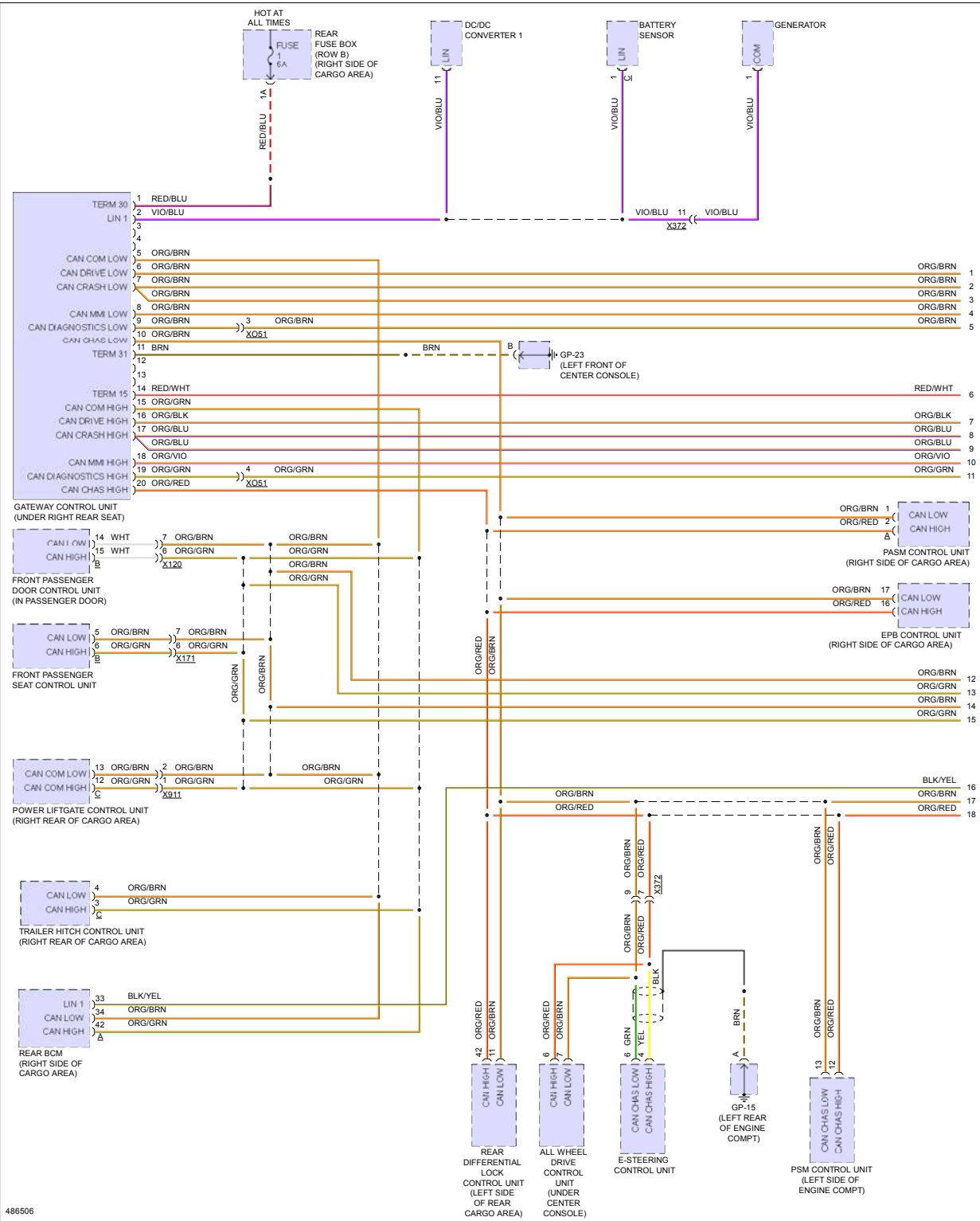
Fig 1: Computer Data Lines Circuit (1 of 3)
