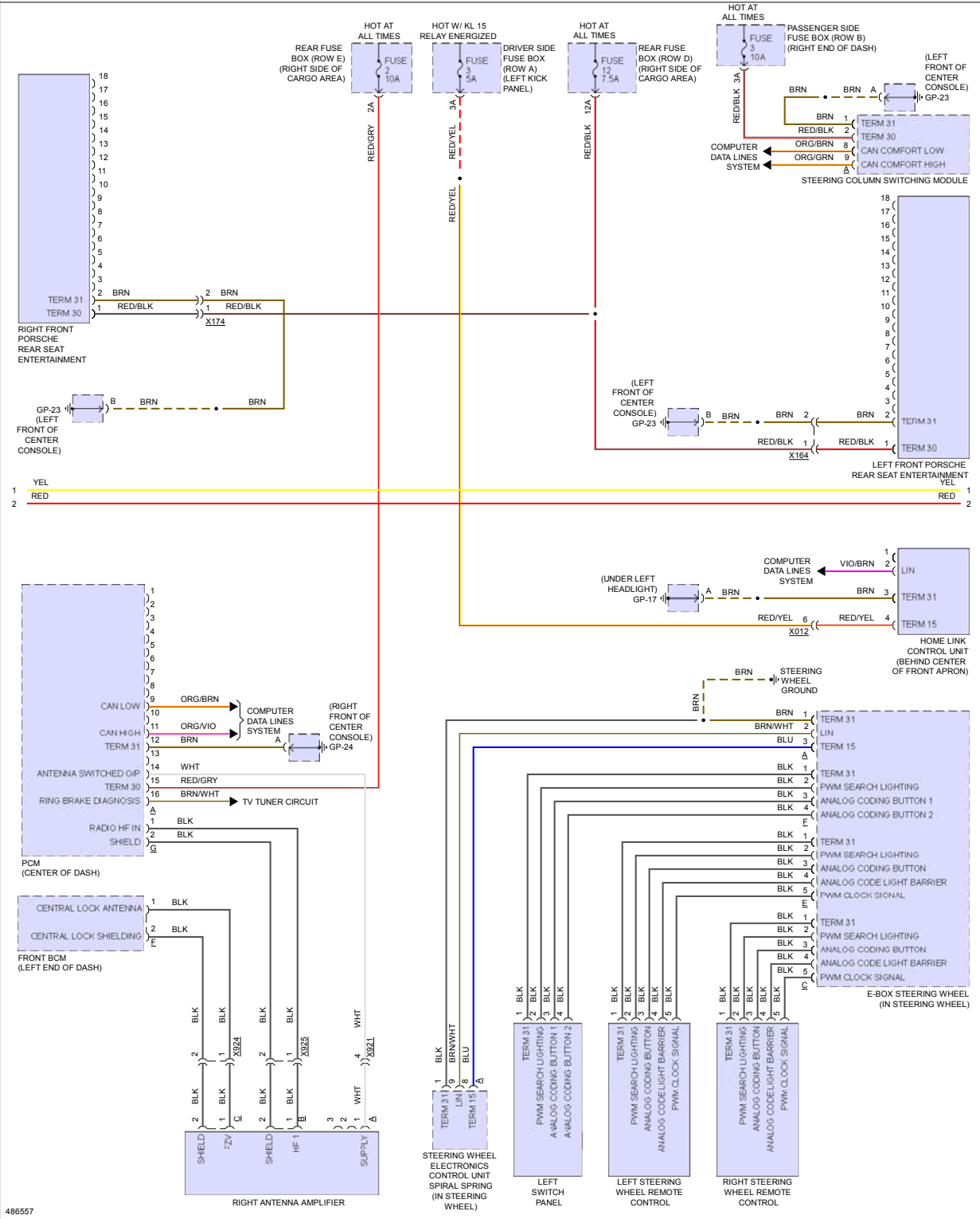
Fig 7: Navigation Circuit, W/ Bose (2 of 3)
