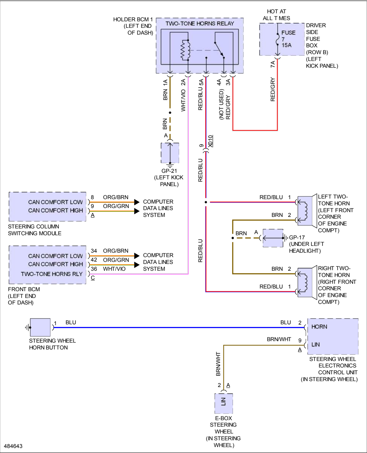
Fig 1: Horn Circuit
