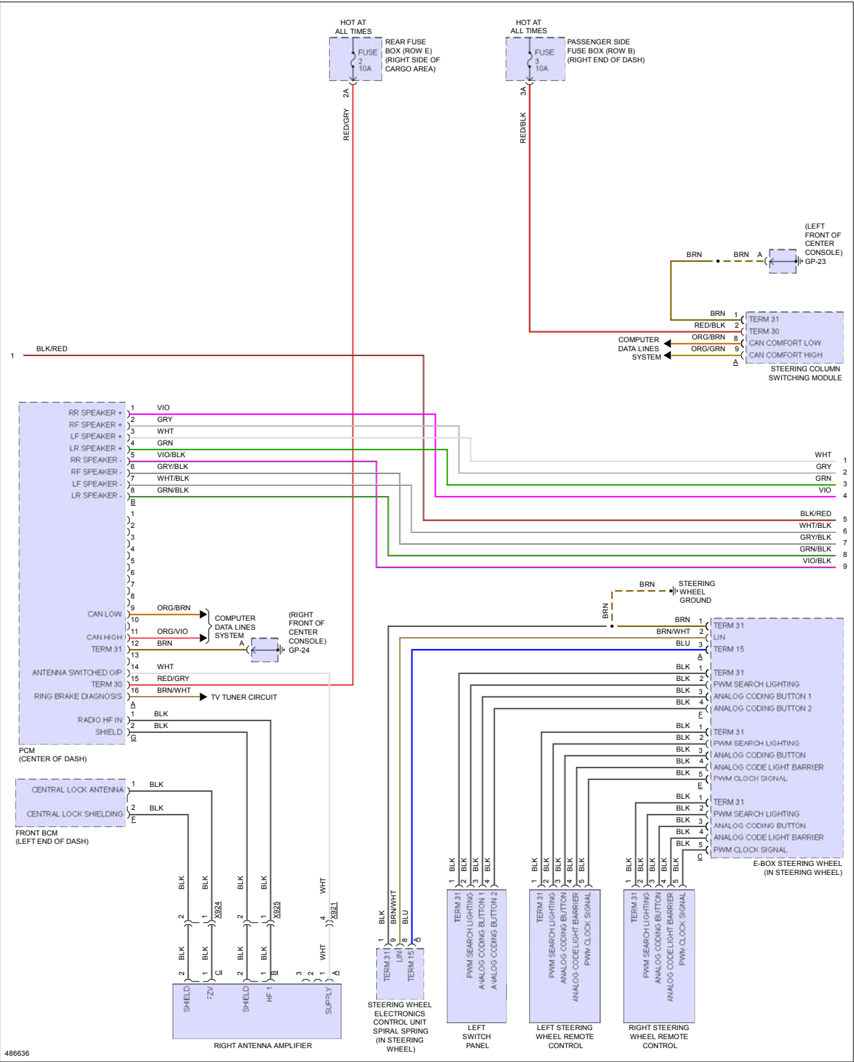
Fig 3: Premium Radio Circuit, W/ ASK (2 of 3)
