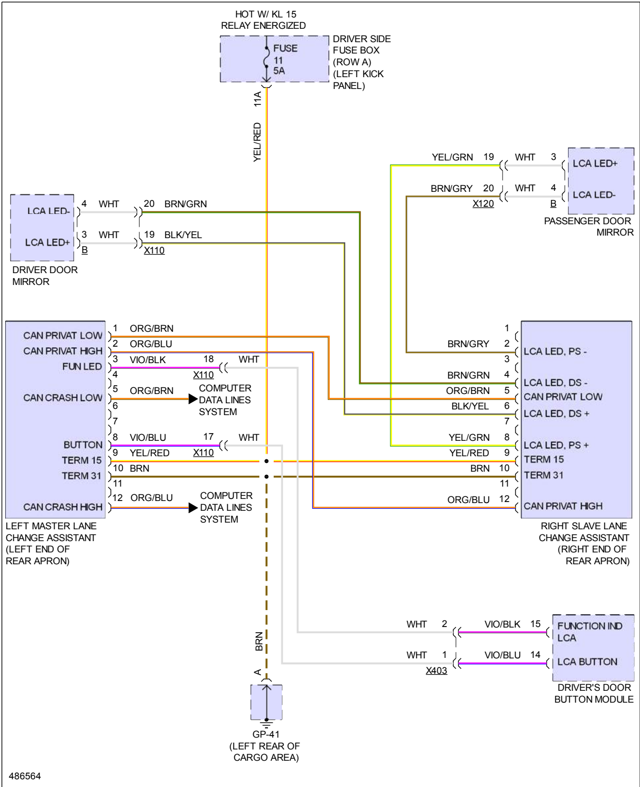
Fig 2: Lane Change Assistance Circuit
