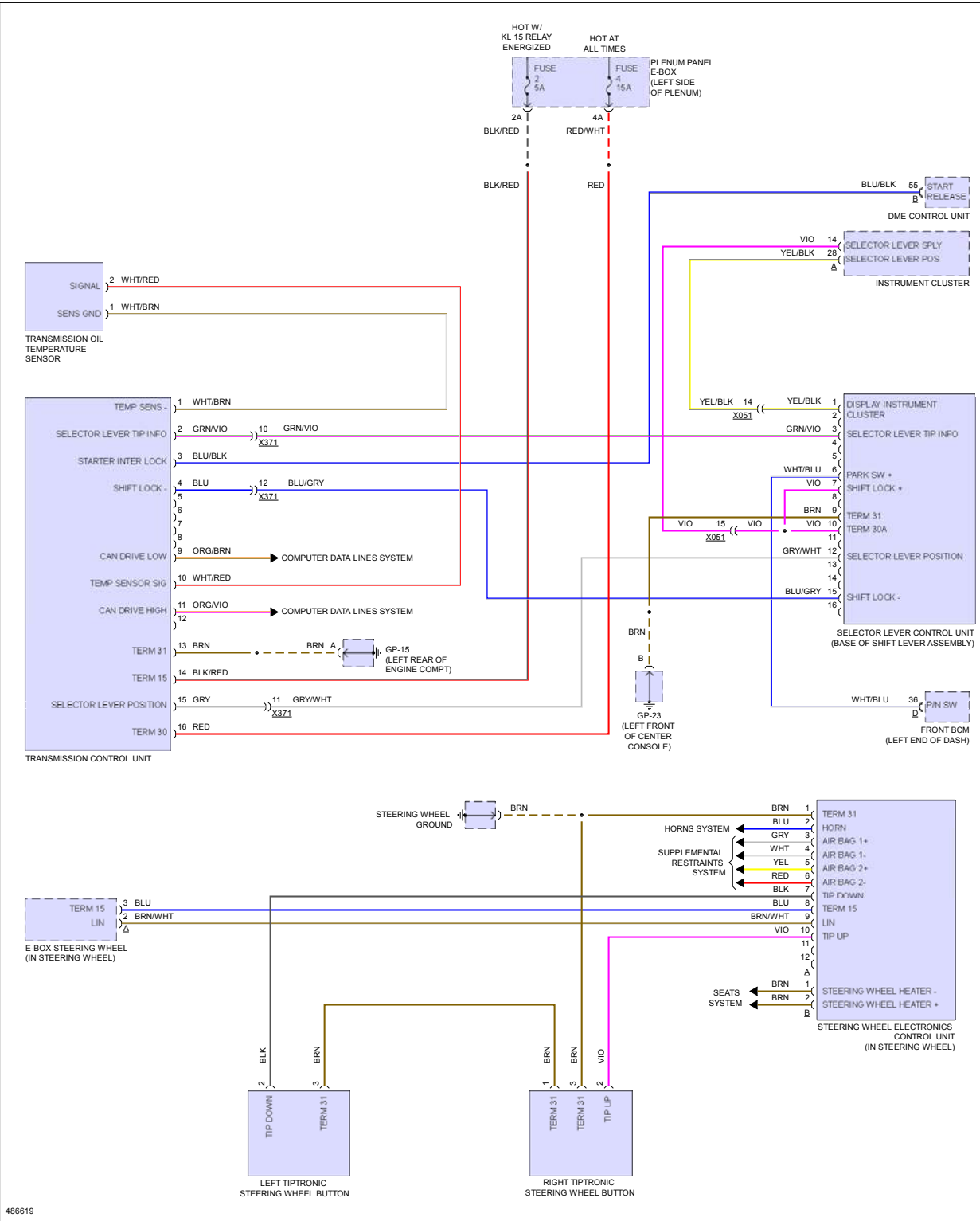
Fig 1: A/T Circuit
