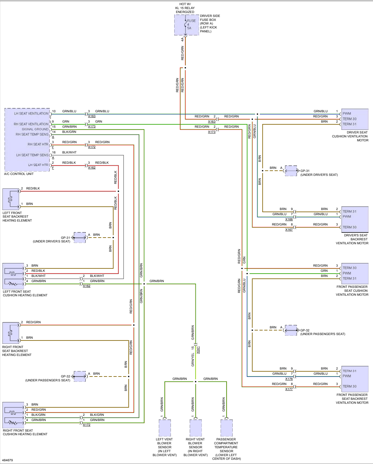
Fig 2: Front Seat Heater Circuit
