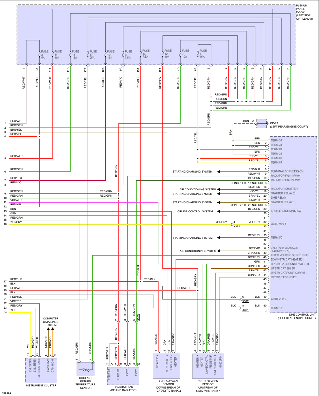
Fig 6: 3.6L Turbo, Engine Performance Circuit (6 of 6)
