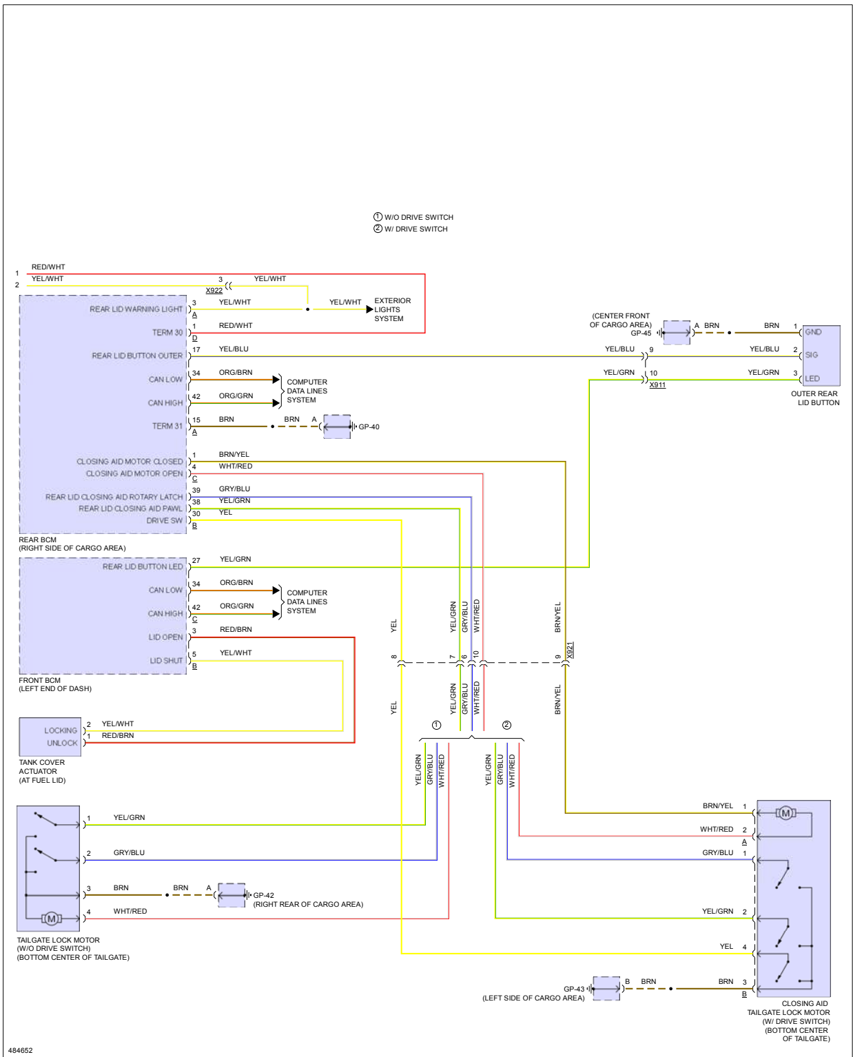
Fig 2: Tailgate & Fuel Door Release Circuit (2 of 2)
