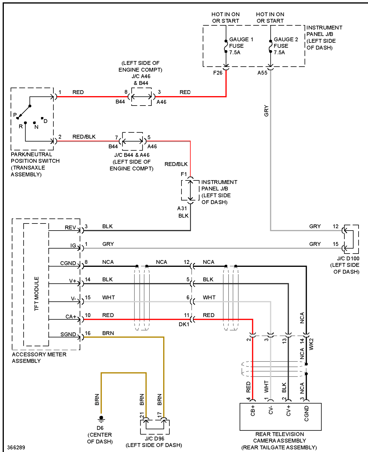
Fig. 67: Rear View Camera Circuit
