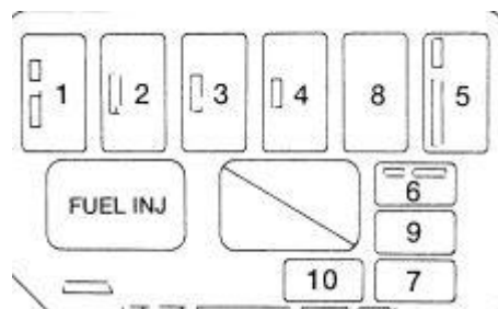
Mercury Tracer – fuse box – engine compartment
