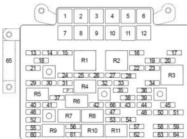
Chevrolet Tahoe – fuse box diagram – engine
