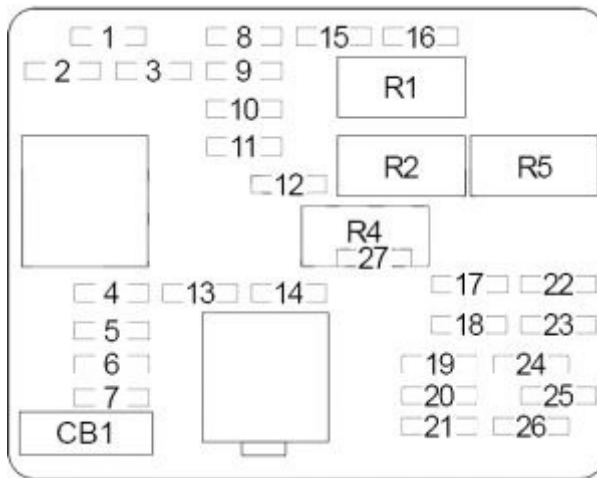
Chevrolet Tahoe – fuse box diagram – passenger
