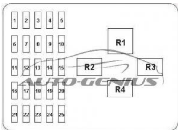
Fiat Doblo – fuse box diagram – instrument panel
