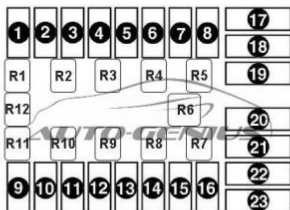
Fiat Doblo – fuse box diagram – engine
