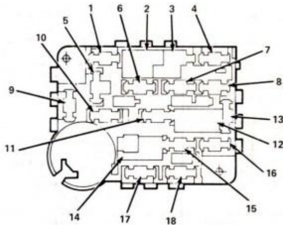
Lincoln Mark VII – fuse box
