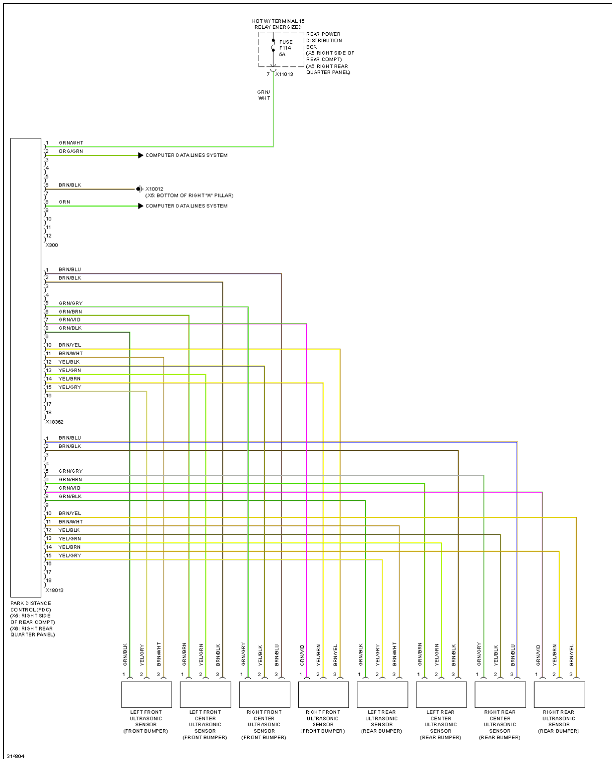
Fig. 79: Parking Assistant Circuit
