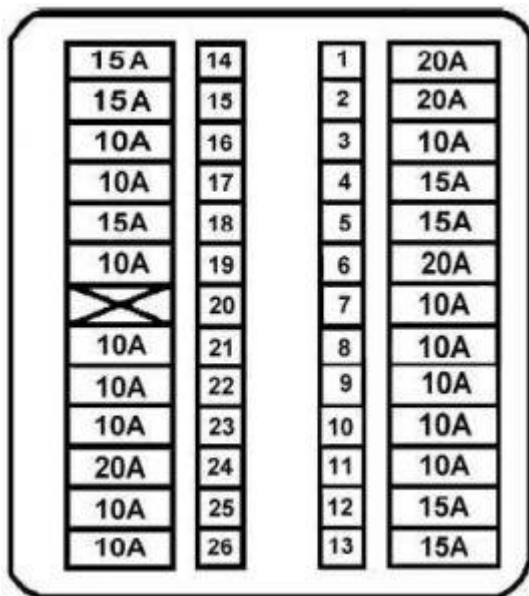
Infiniti G20 – fuse box diagram – passenger
