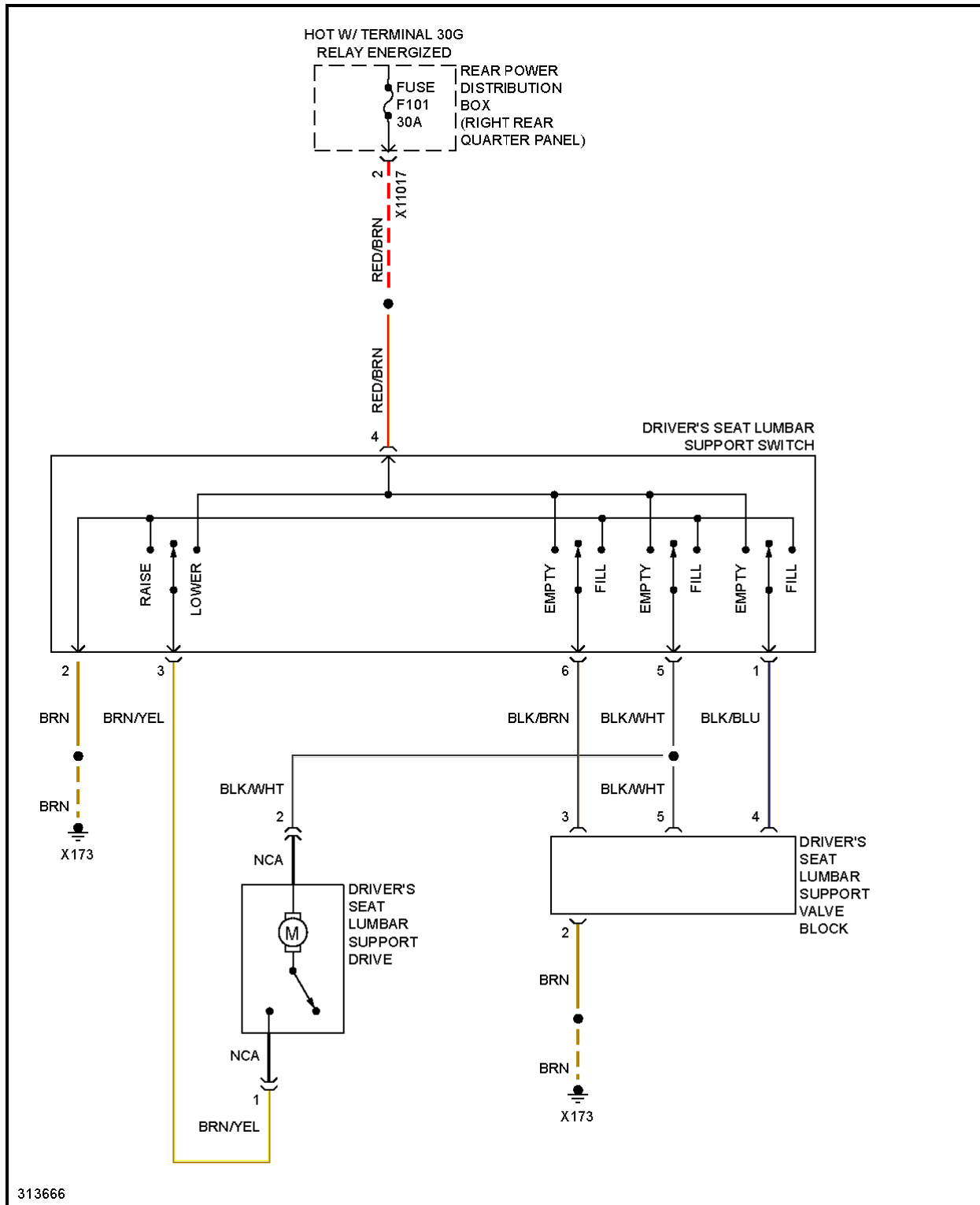
Fig. 89: Driver's Lumbar Circuit
