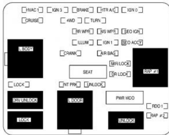
GMC Yukon – fuse box – instrument panel
