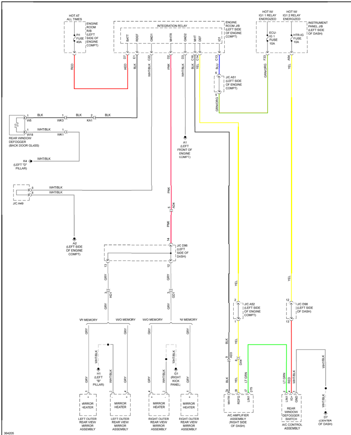
Fig. 27: Mirror Heater & Rear Defogger Circuit
