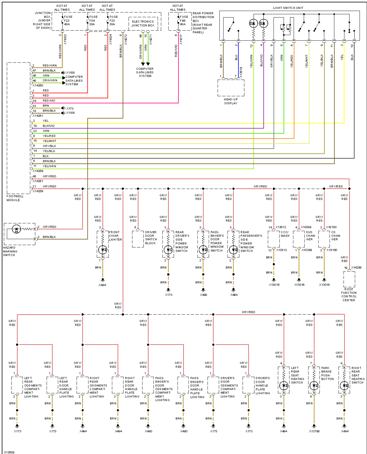
Fig. 58: Instrument Illumination Circuit
