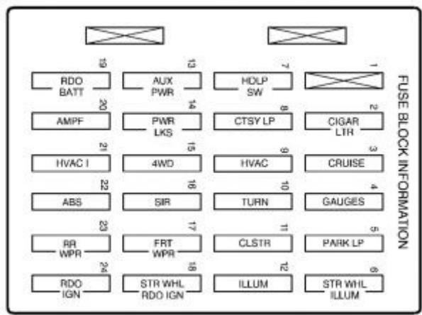
GMC Envoy mk1 – fuse box – instrument panel
