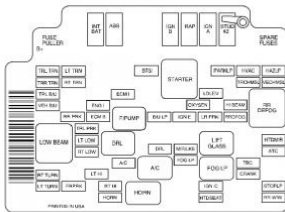
GMC Envoy mk1 – fuse box – engine
