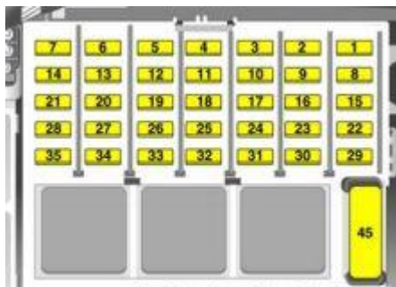
Vauxhall Combo C – fuse box – engine Z13DTJ
