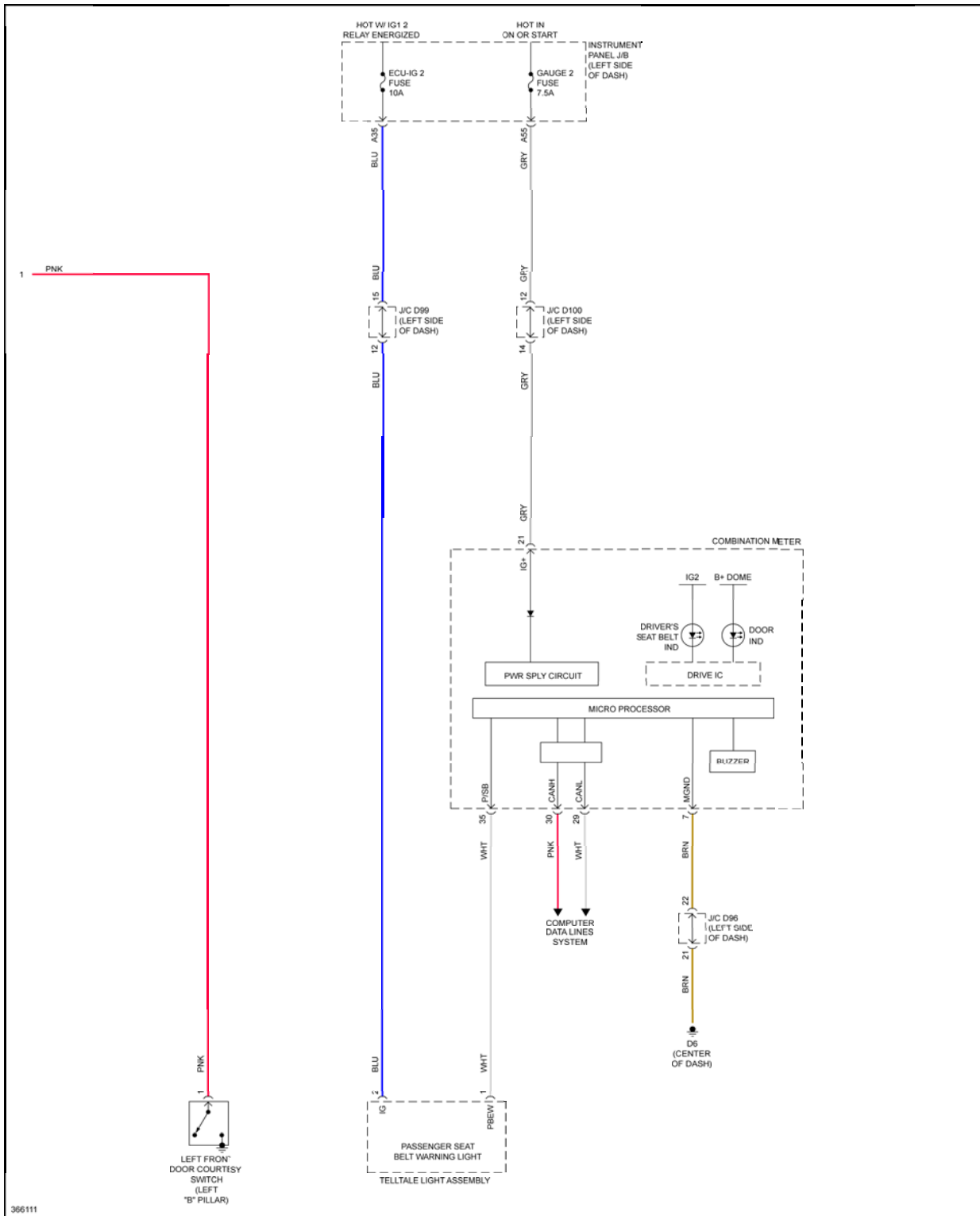
Fig. 124: Key Reminder & Seat Belt Warning Circuit (2 of 2)
