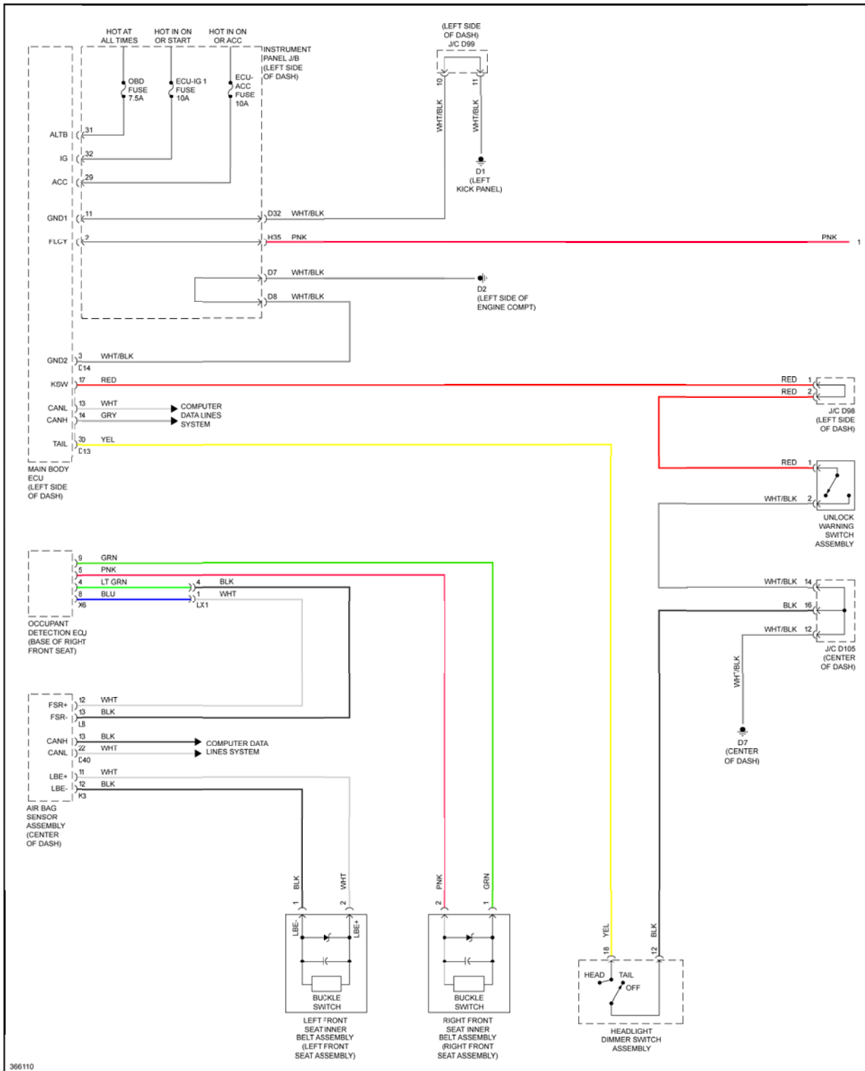
Fig. 123: Key Reminder & Seat Belt Warning Circuit (1 of 2)
