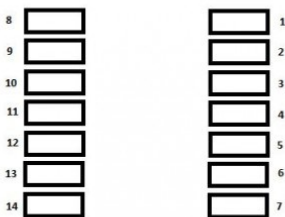
Citroen C1 mk1 – fuse box – under dashboard
