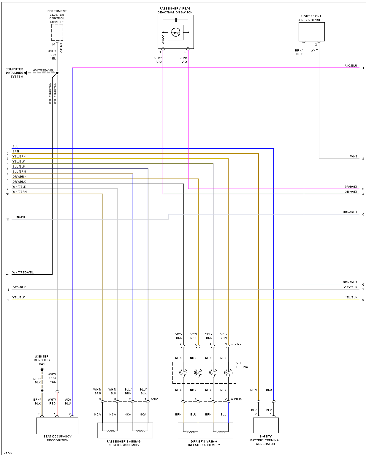
Fig. 66: Supplemental Restraints Circuit (2 of 3)
