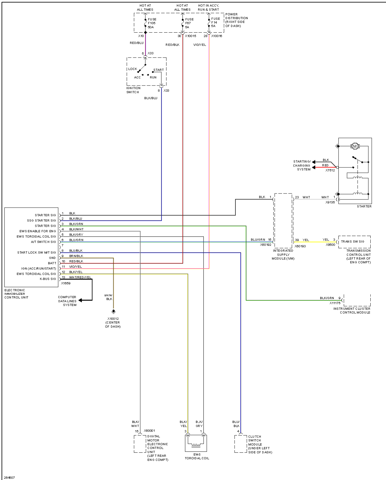
Fig. 8: Immobilizer Circuit
