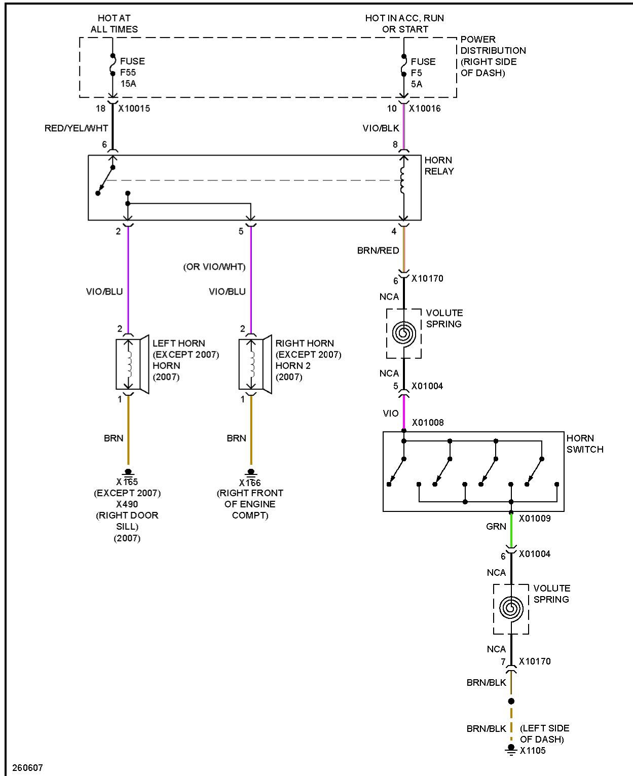
Fig. 30: Horn Circuit
