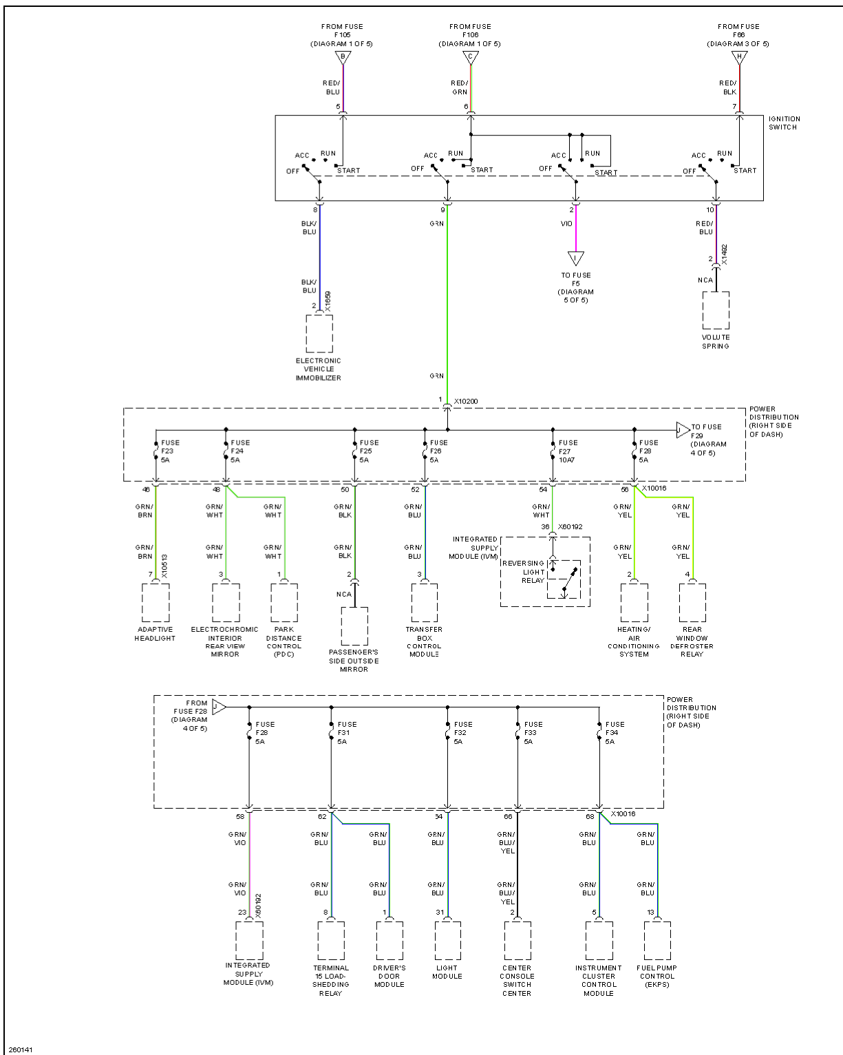
Fig. 42: Power Distribution Circuit (4 of 5)
