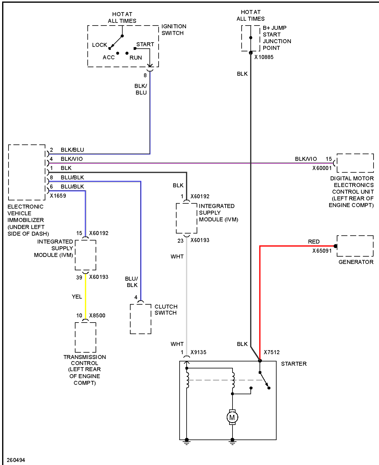
Fig. 64: Starting Circuit
