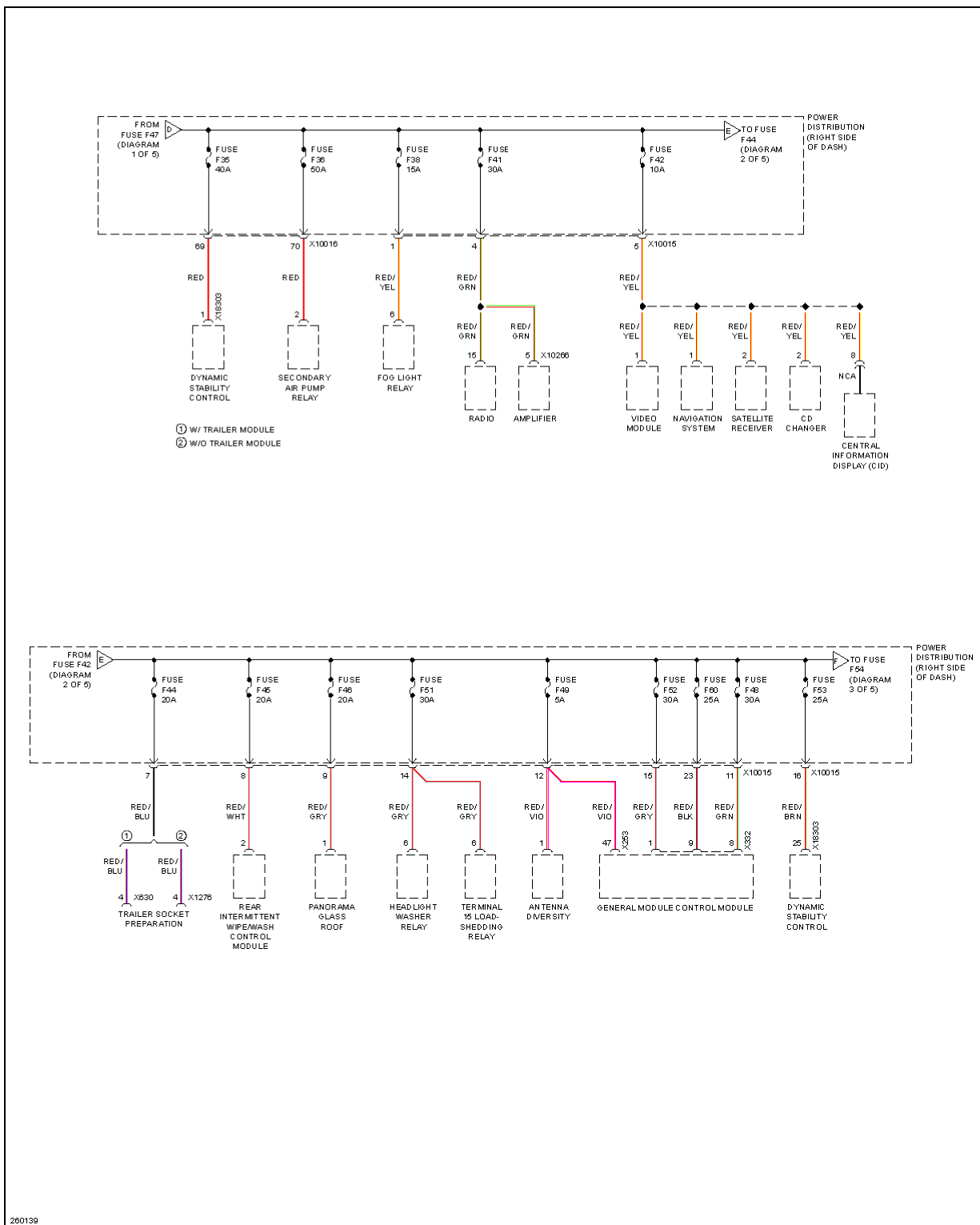
Fig. 40: Power Distribution Circuit (2 of 5)
