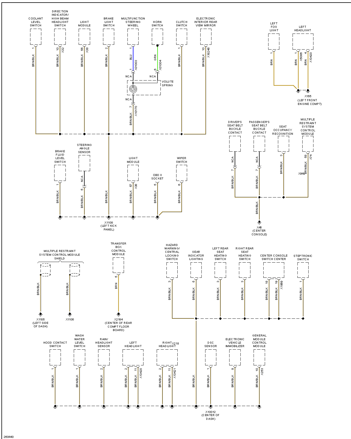
Fig. 24: Ground Distribution Circuit (2 of 4)
