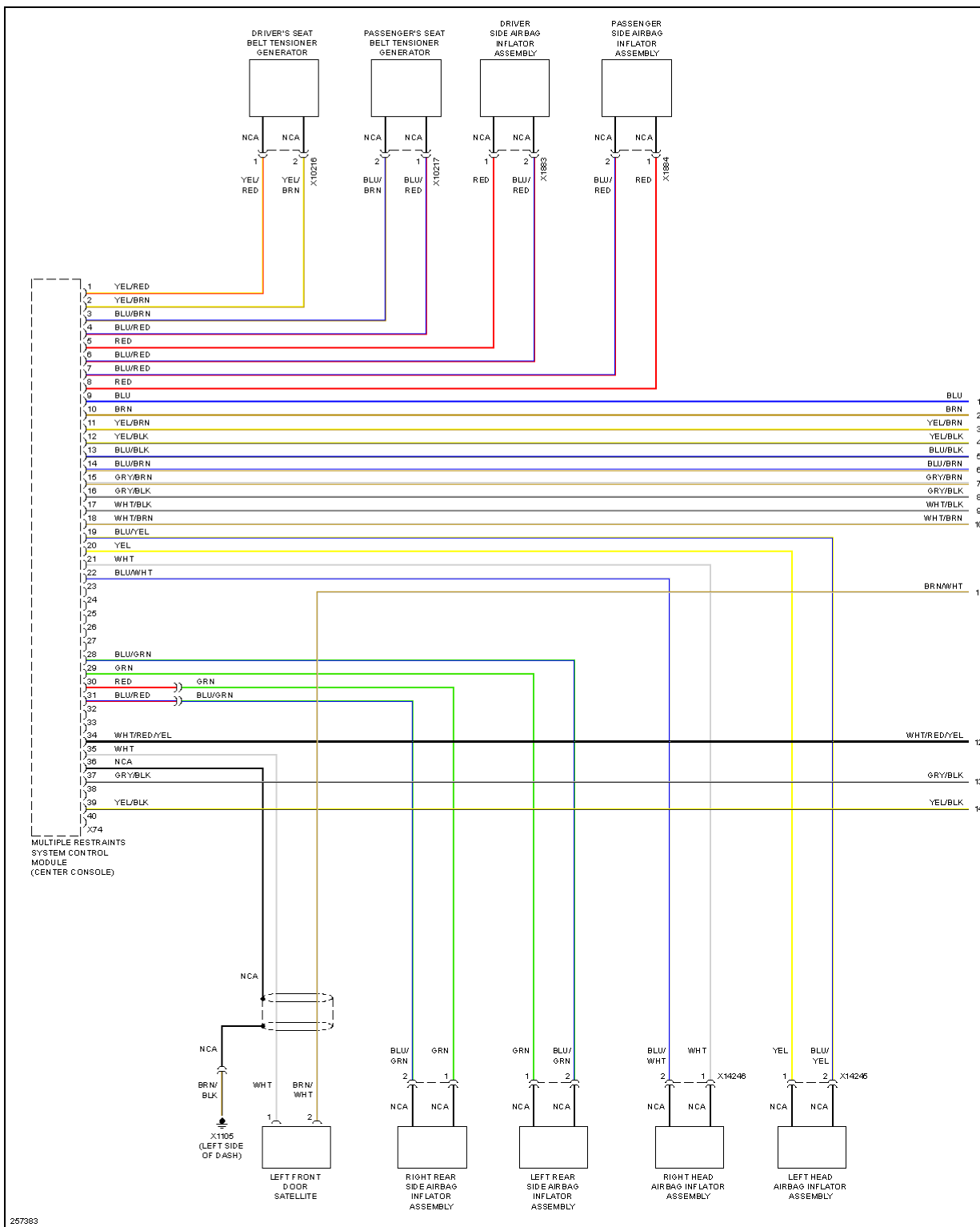
Fig. 65: Supplemental Restraints Circuit (1 of 3)
