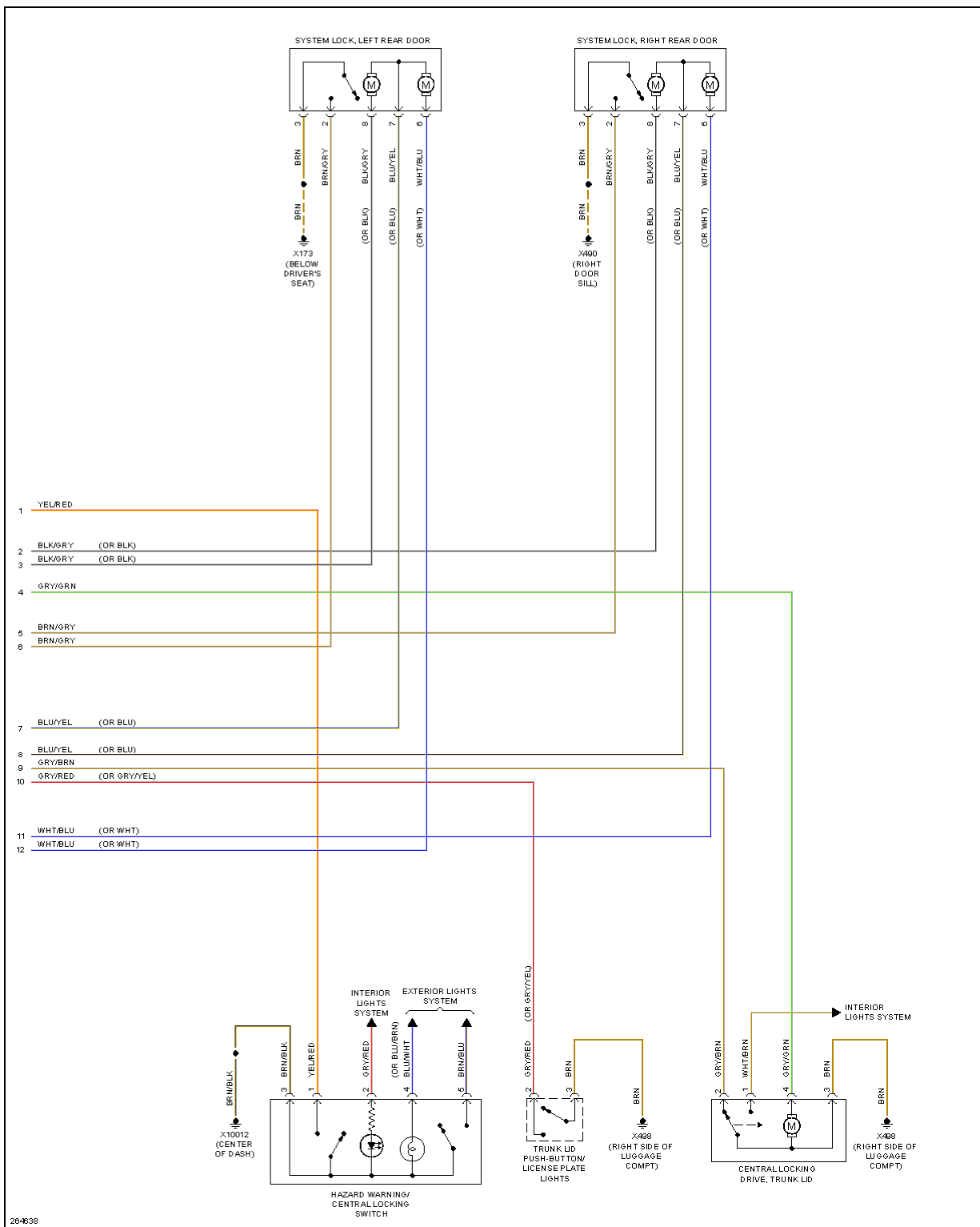
Fig. 45: Power Door Locks Circuit (2 of 2)
