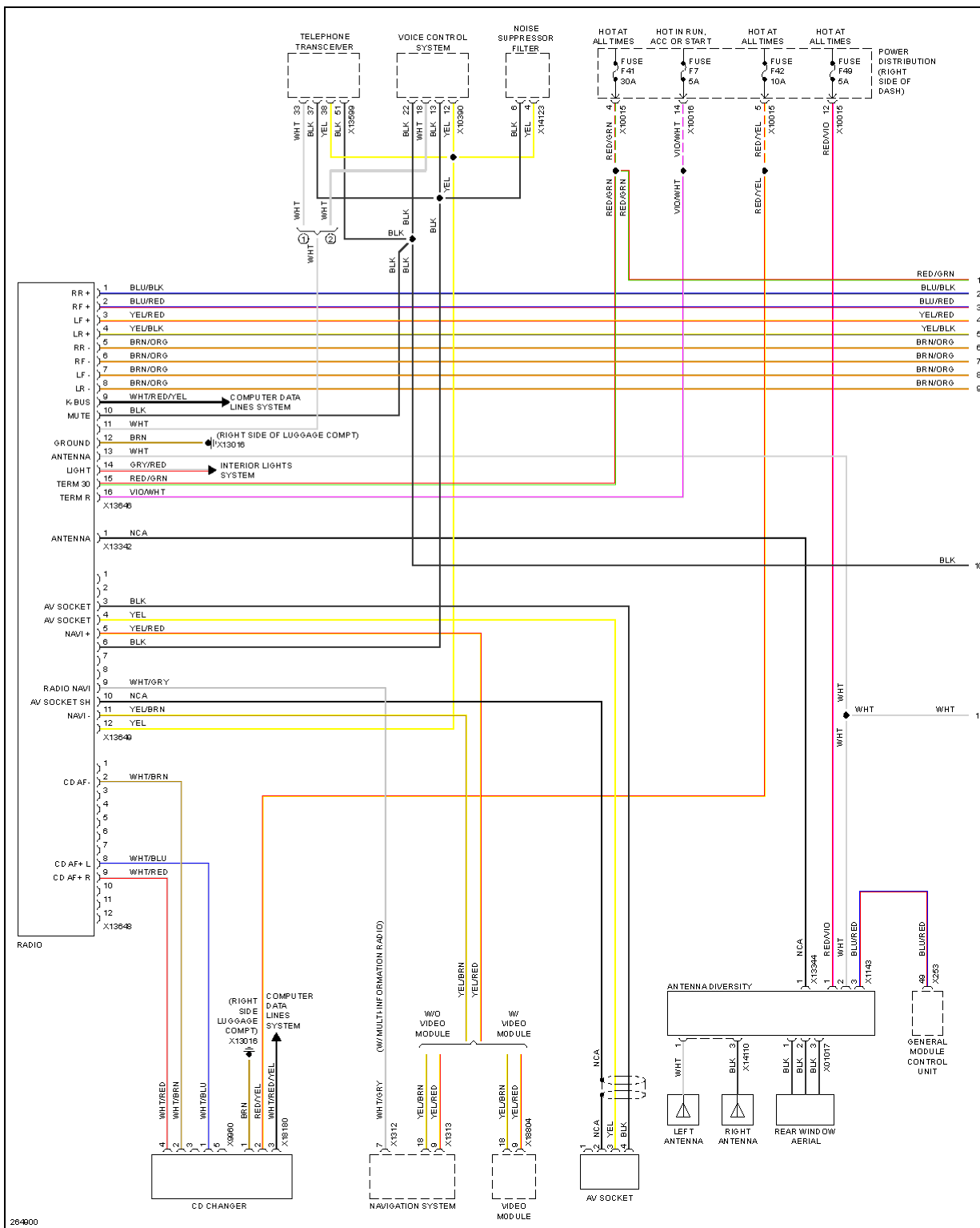
Fig. 58: Premium Radio Circuit, HIFI Radio (1 of 2)
