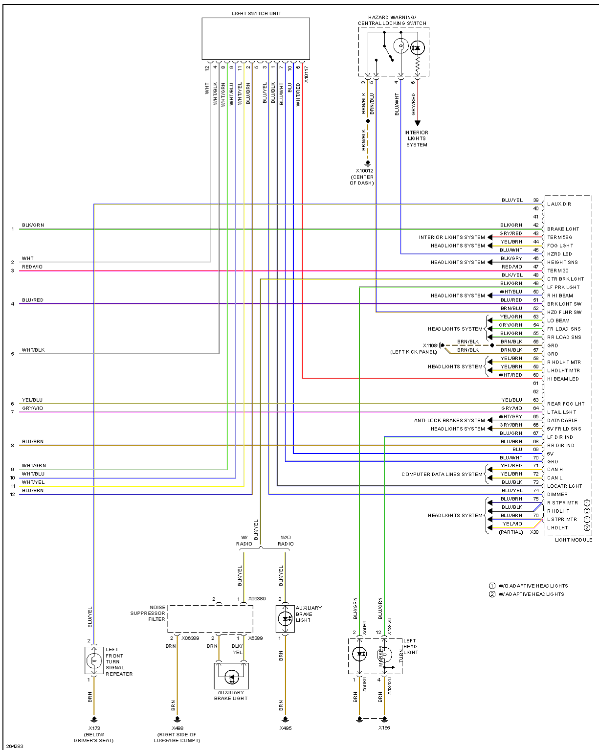
Fig. 22: Exterior Lamps Circuit (3 of 3)
