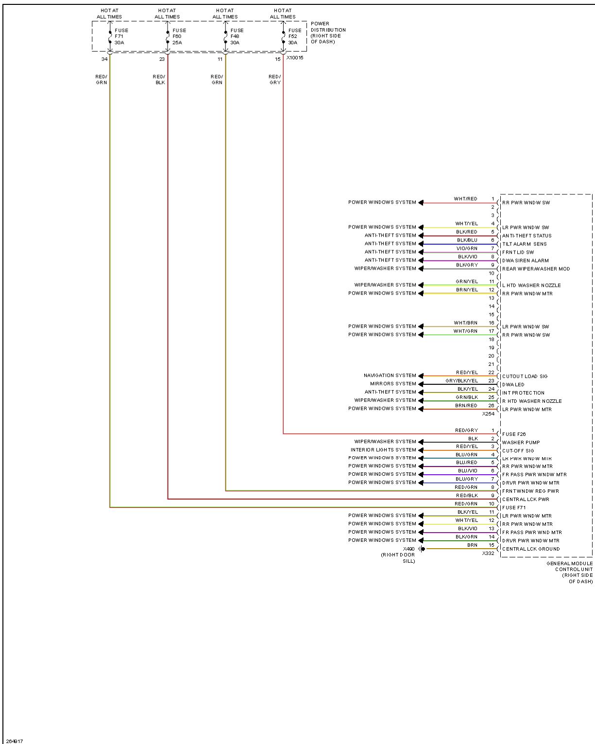
Fig. 10: Body Control Modules Circuit (2 of 2)
