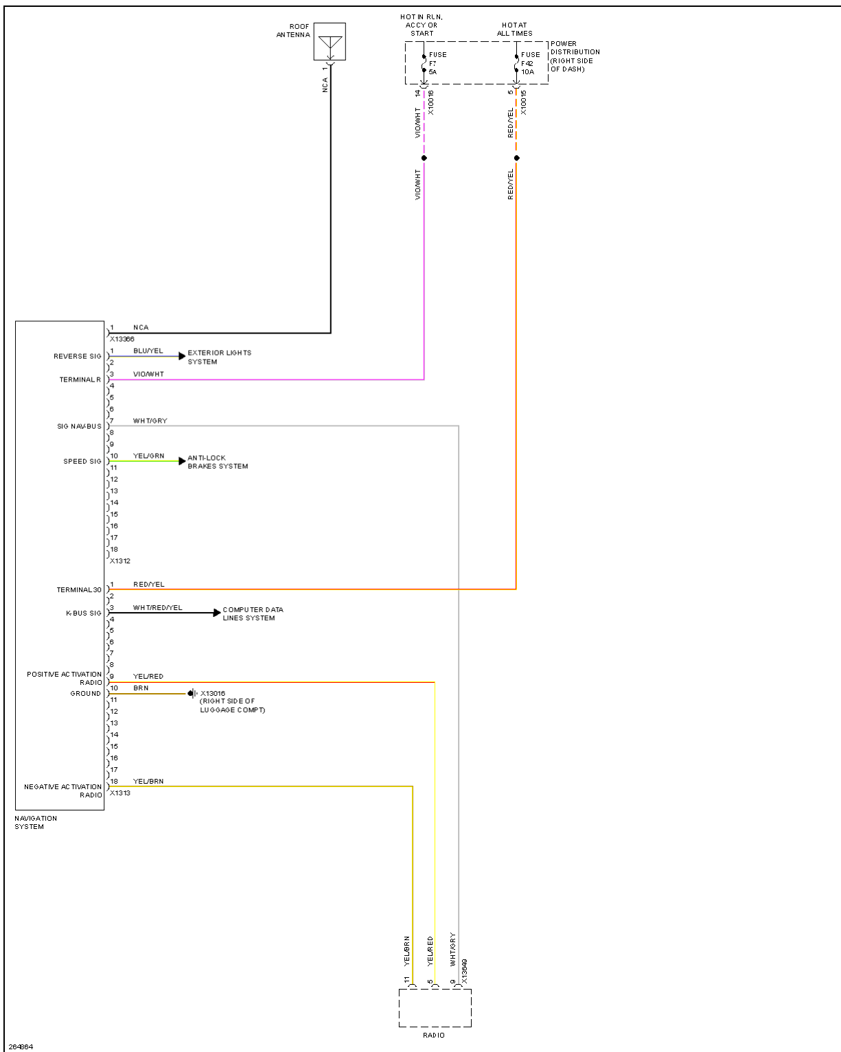
Fig. 35: Navigation Circuit, W/ Multi-Information Radio
