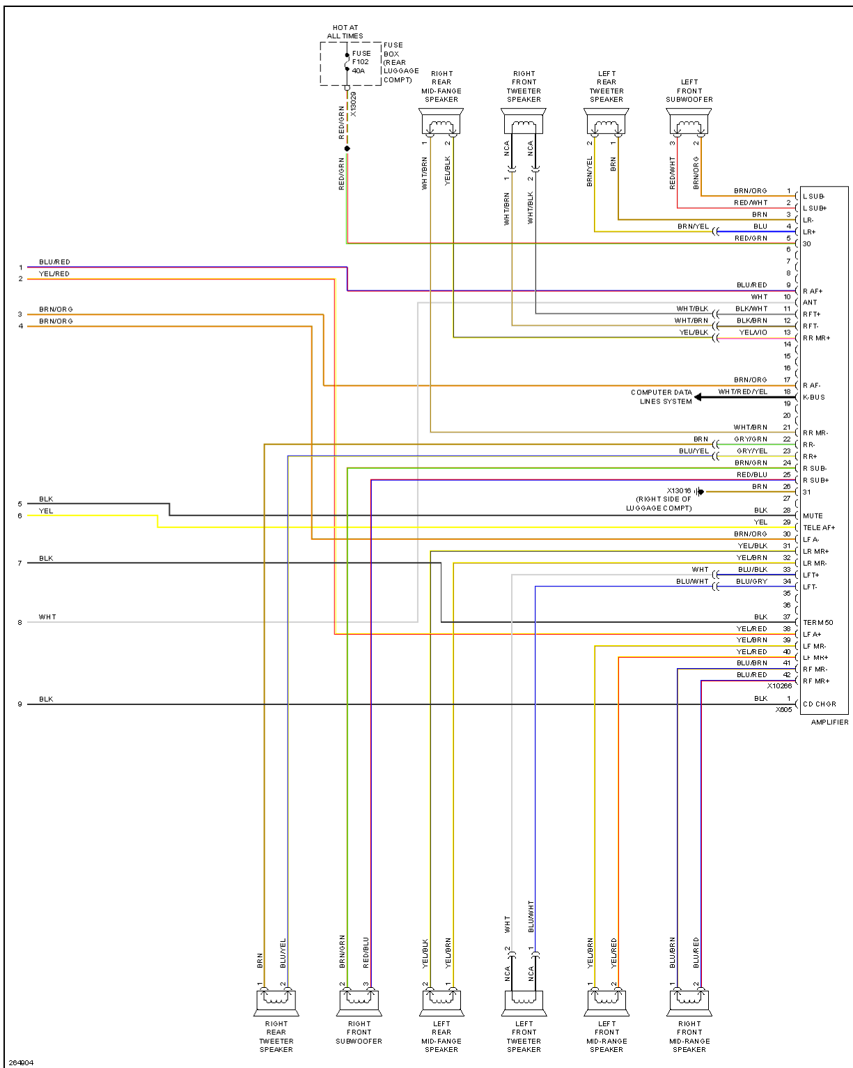
Fig. 61: Premium Radio Circuit, Top HIFI Radio (2 of 2)
