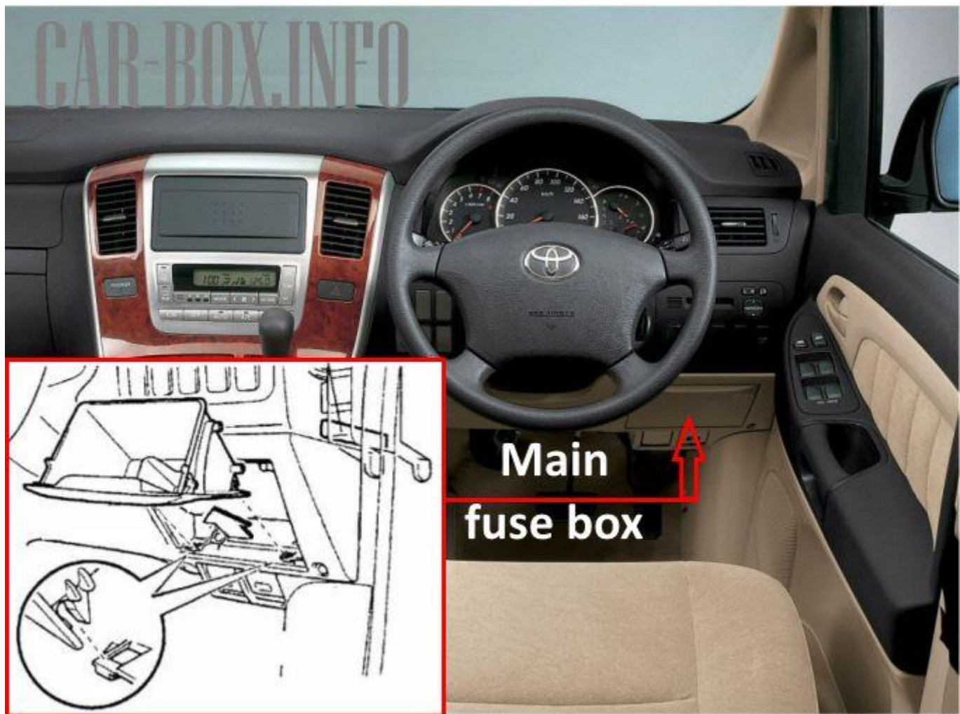
1 - main from the driver's side behind the glove box;
