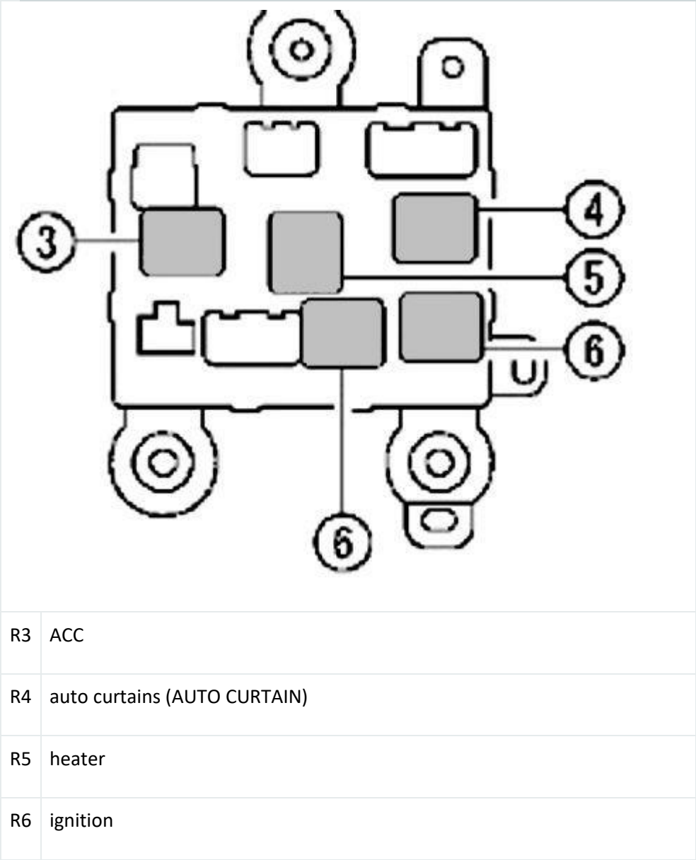
Additional fuse box
