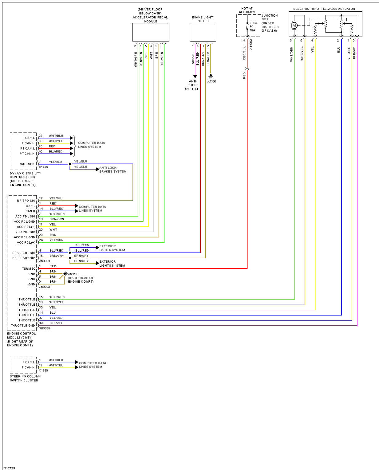
Fig. 22: 3.0L Twin Turbo, Cruise Control Circuit
