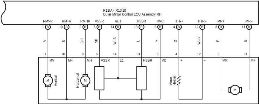
R7 Outer Rear View Mirror Assembly RH
