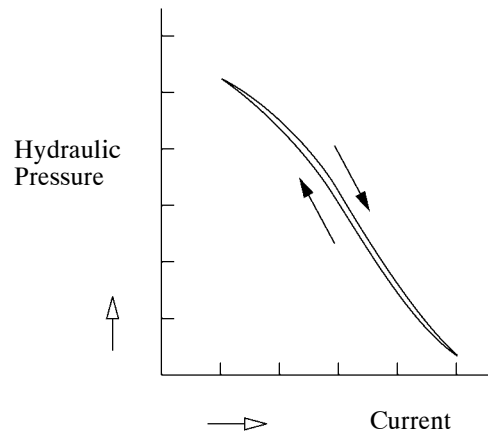
Solenoid Valve SL1, SL2 and SLT
