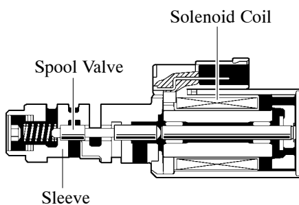
Solenoid Valve SLU
