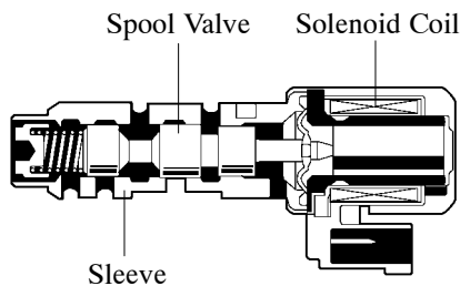
Solenoid Valve SL1, SL2
