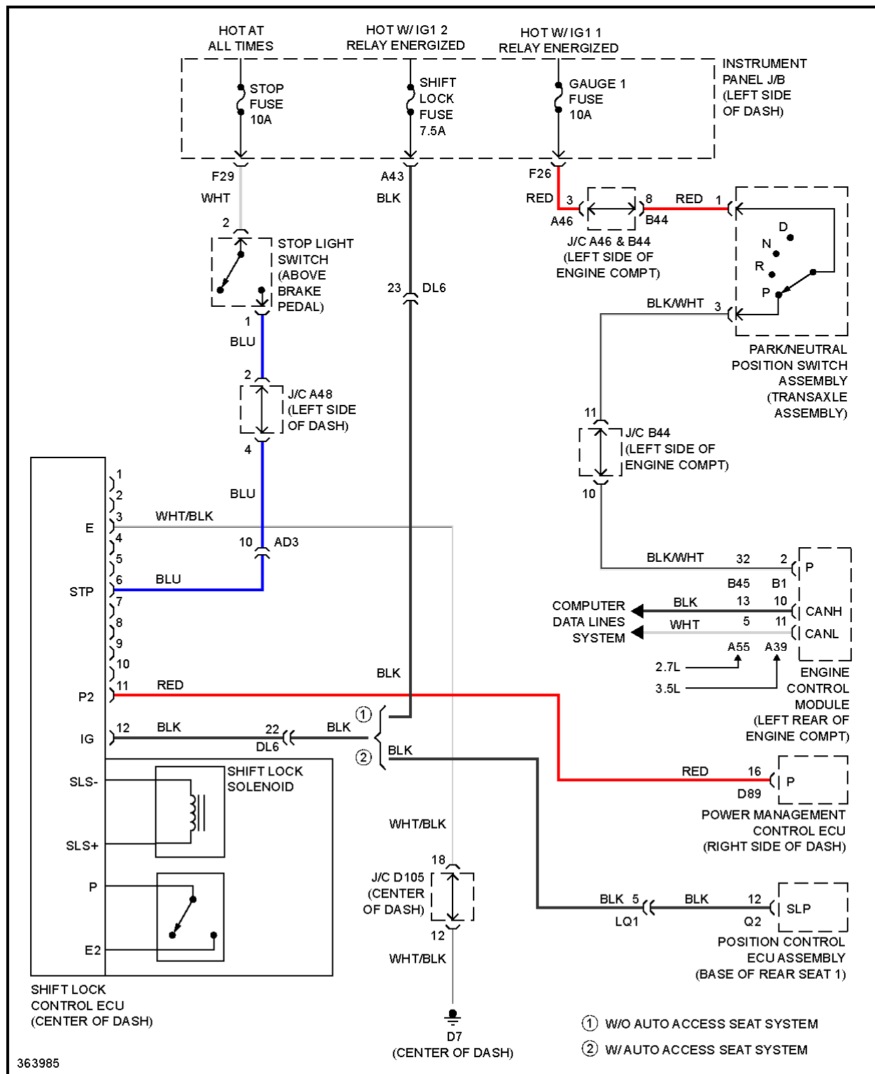
Fig. 102: Shift Interlock Circuit, W/ Smart Key System
