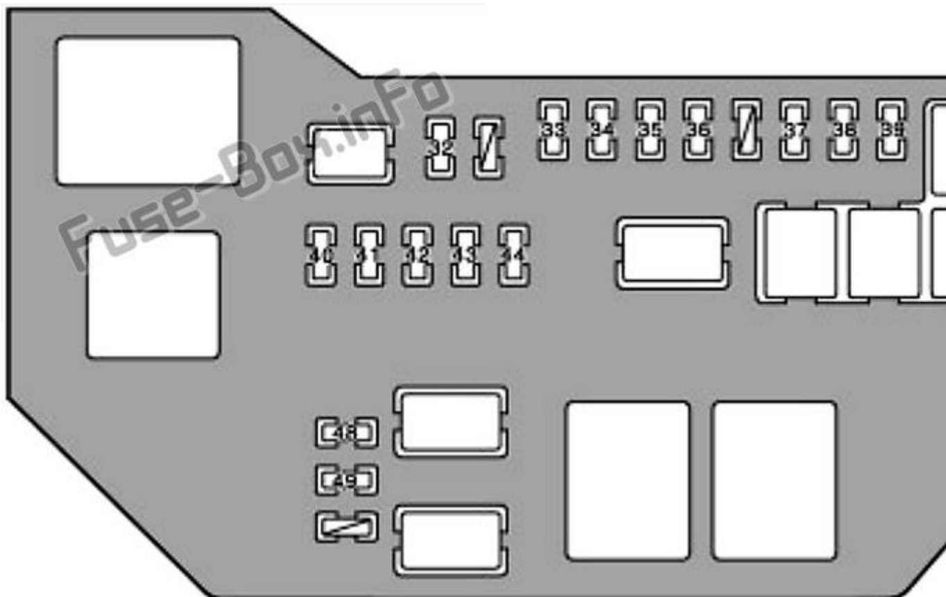
Assignment of the fuses in the engine compartment (2003-2005)
