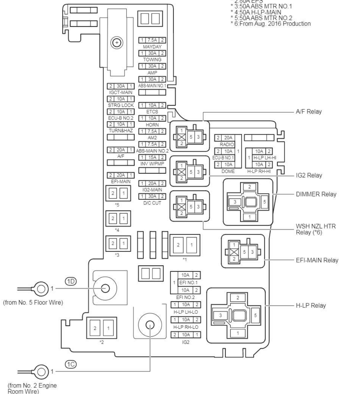
Top View
