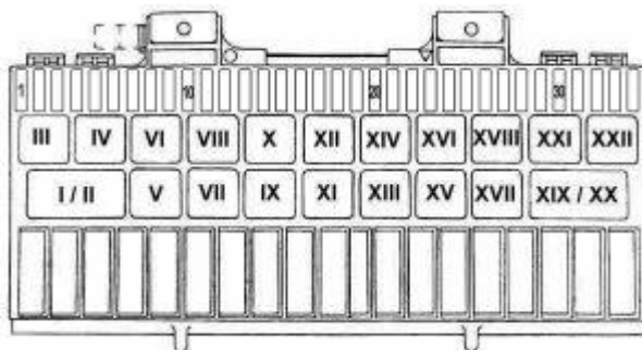
Porsche 928 – fuse box diagram
