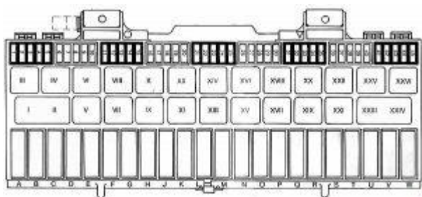
Porsche 928 – fuse box diagram
