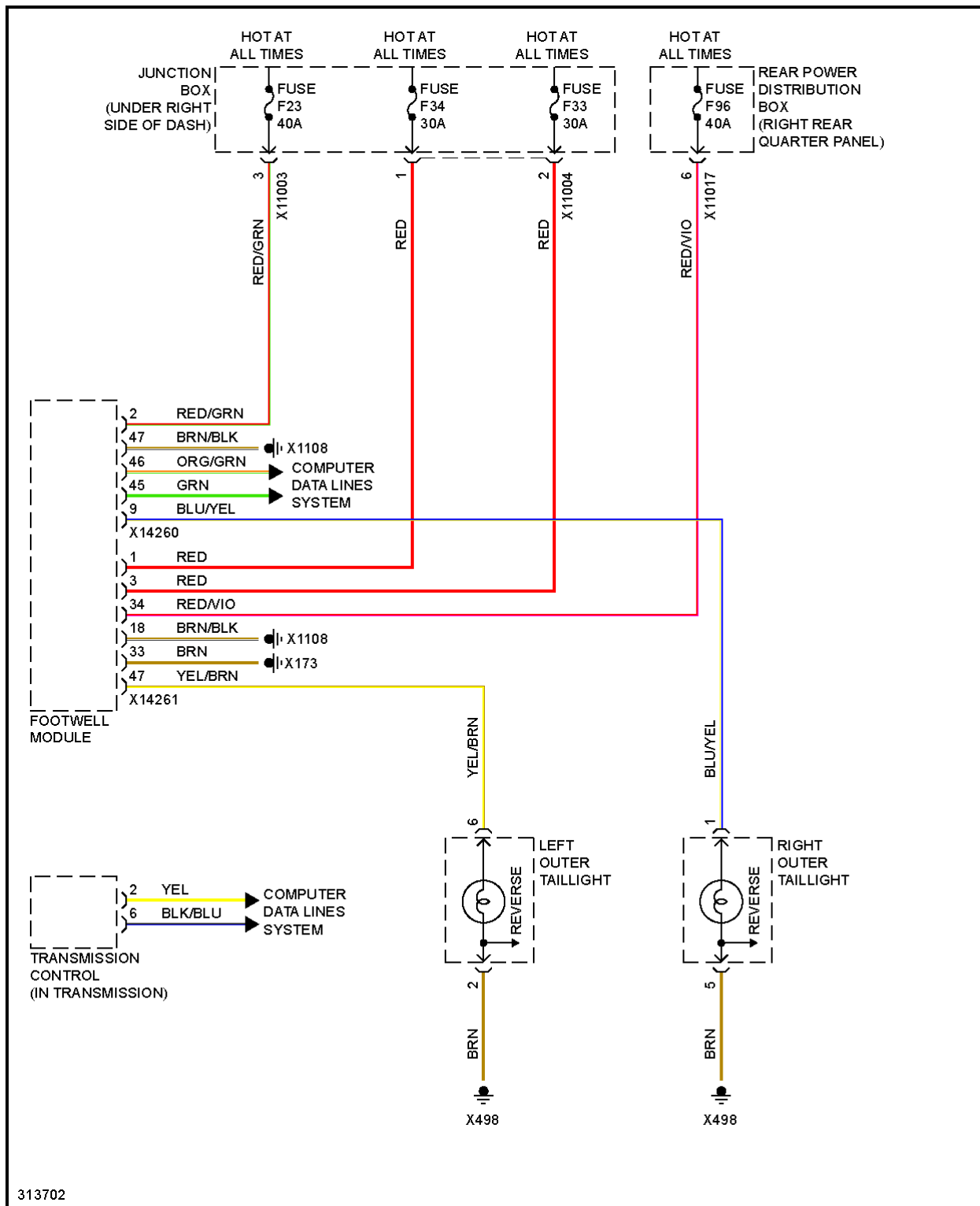
Fig. 41: Backup Lamps Circuit
