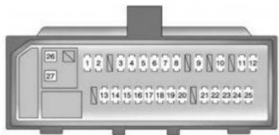
Pontiac Vibe – fuse box – instrument
