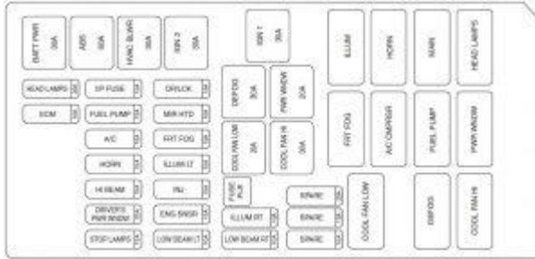
Suzuki Forenzo – fuse box diagram –
