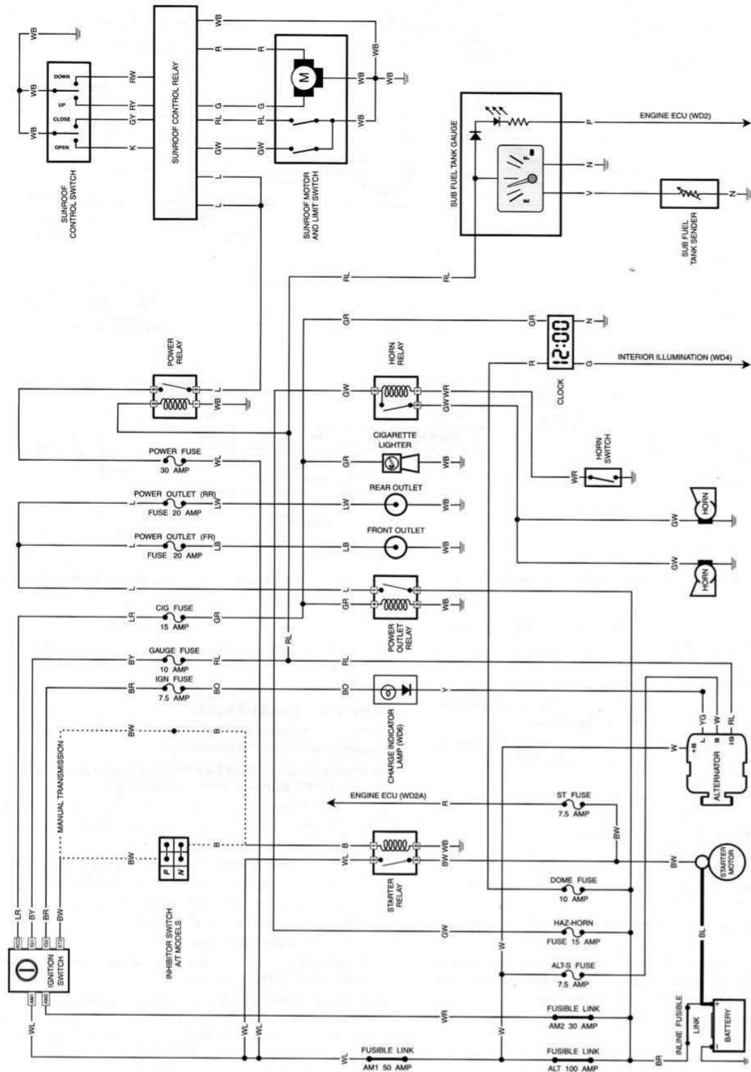
Starting, charging, clock, power outlets, horn and sunroof. Early models.
