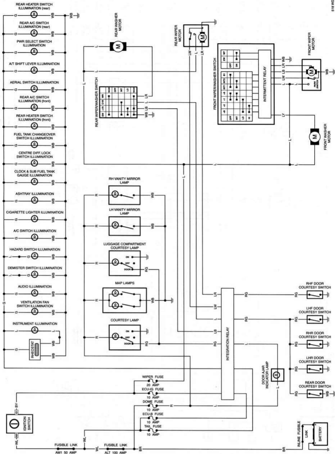
Interior illumination, front and rear wiper/washers. Late models
