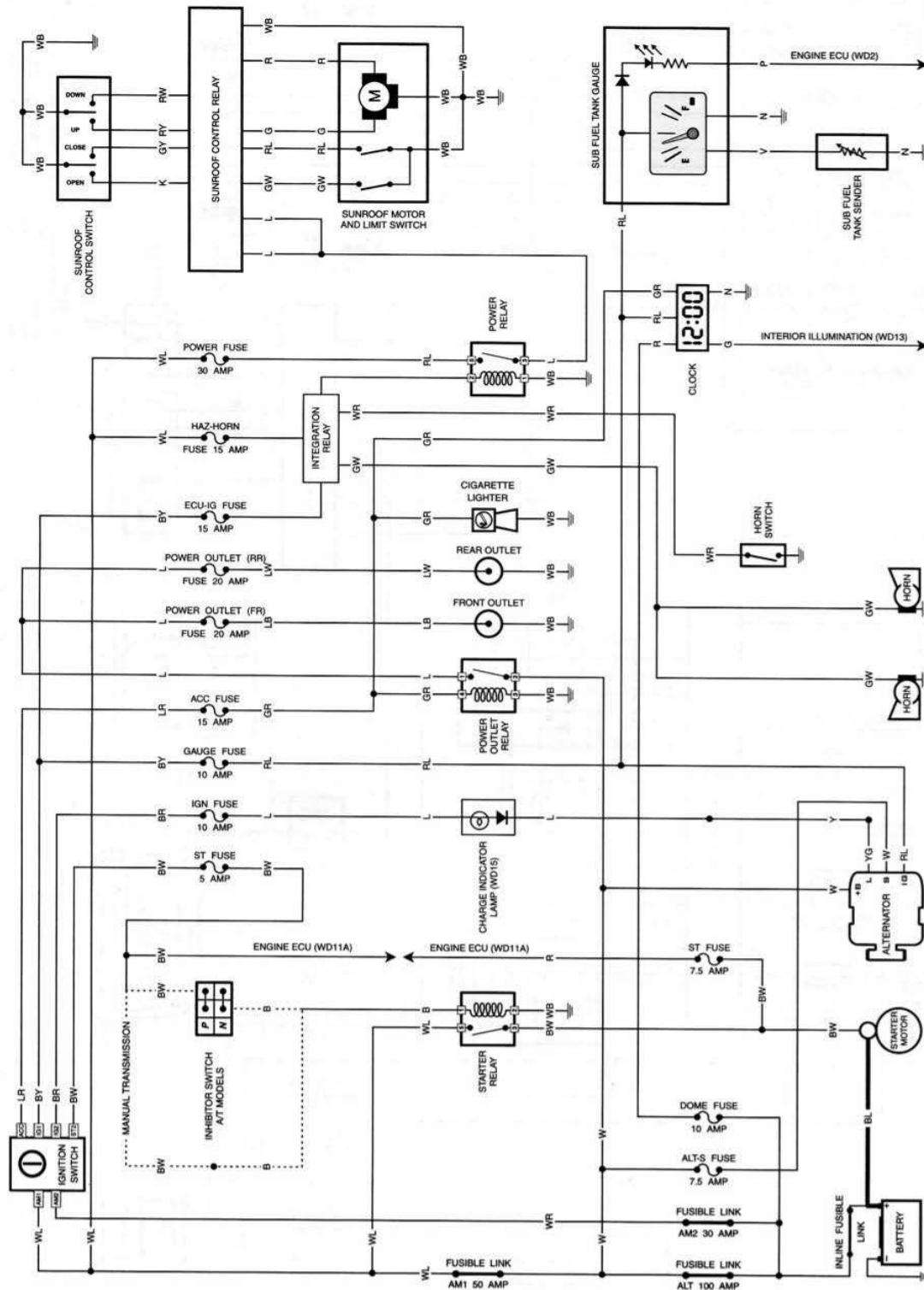
Starting, charging, clock, cigarette lighter, power outlets, horn and sunroof. Late models.
