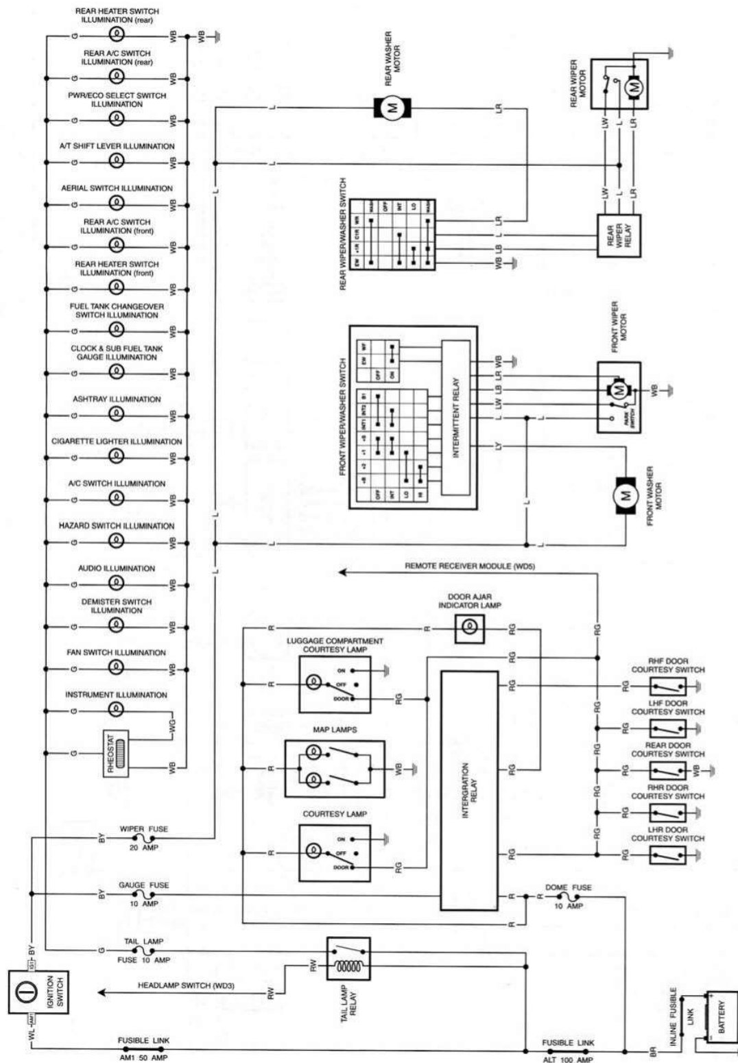
Interior illumination, front and rear wiper/washers. Early models.
