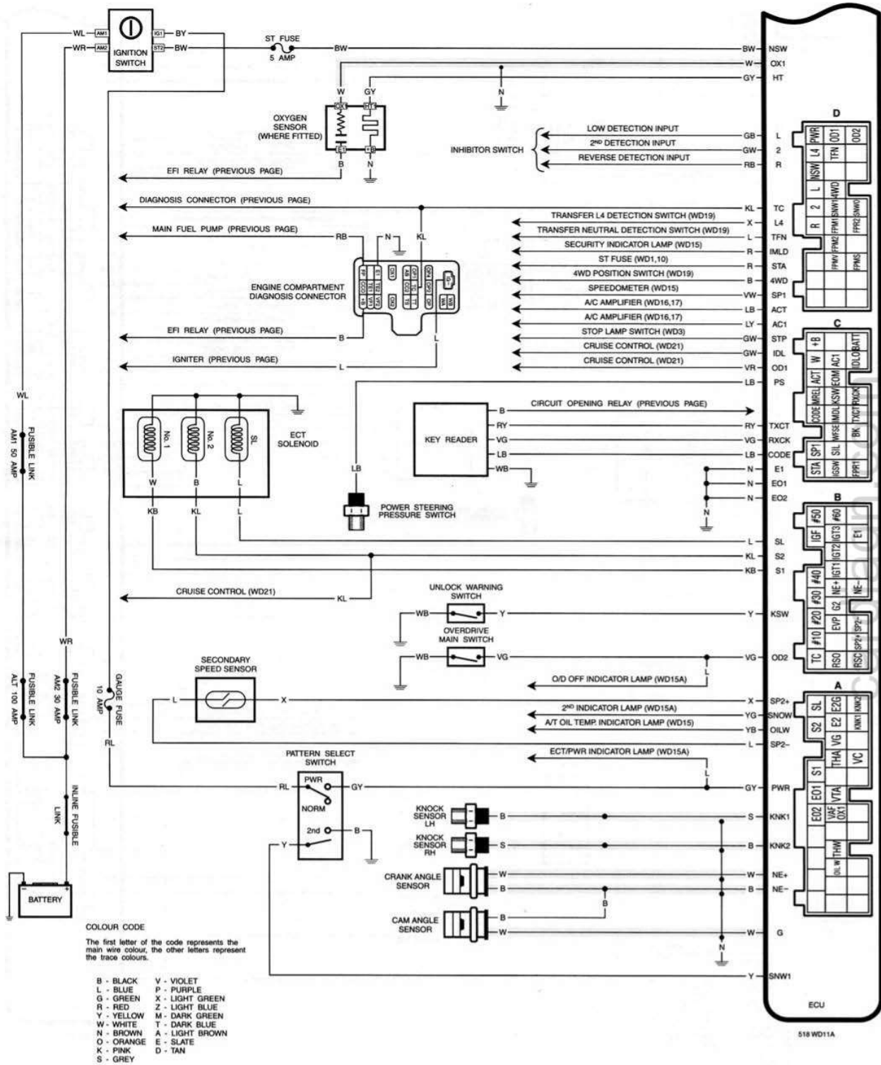
Fuel and engine management system. Late models.
