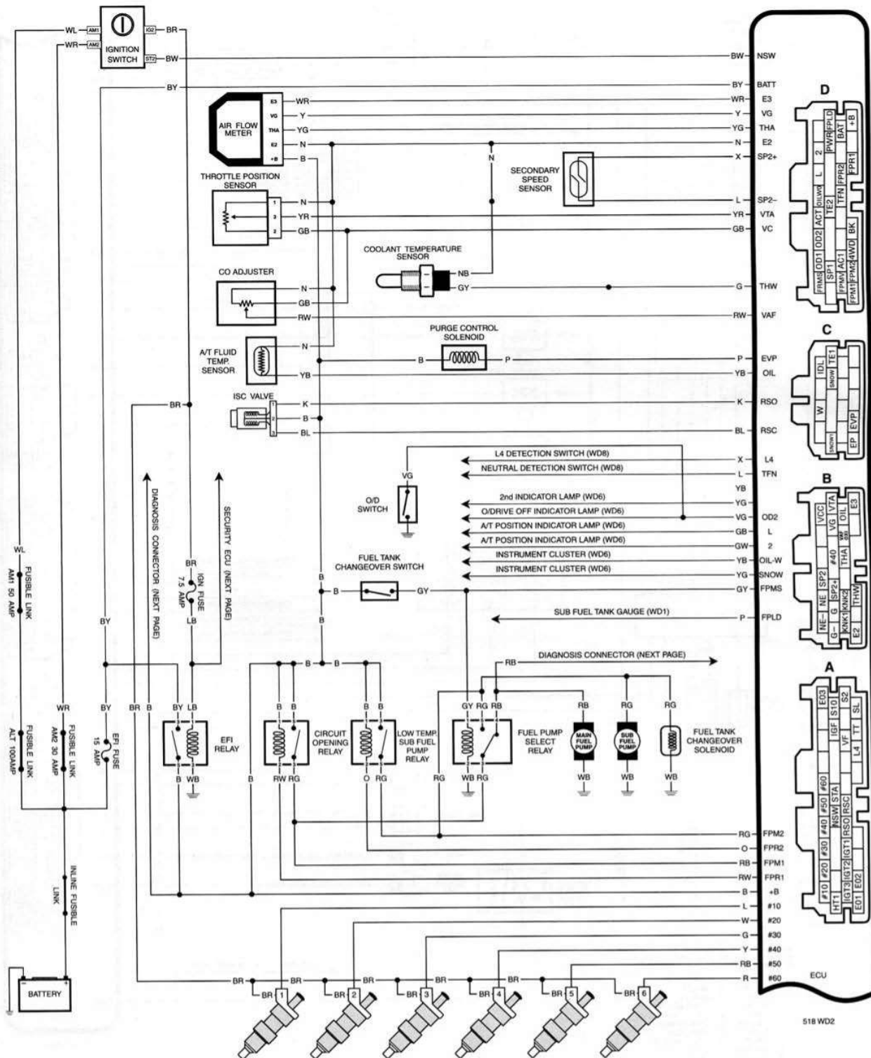
Fuel and engine management. Early models.
