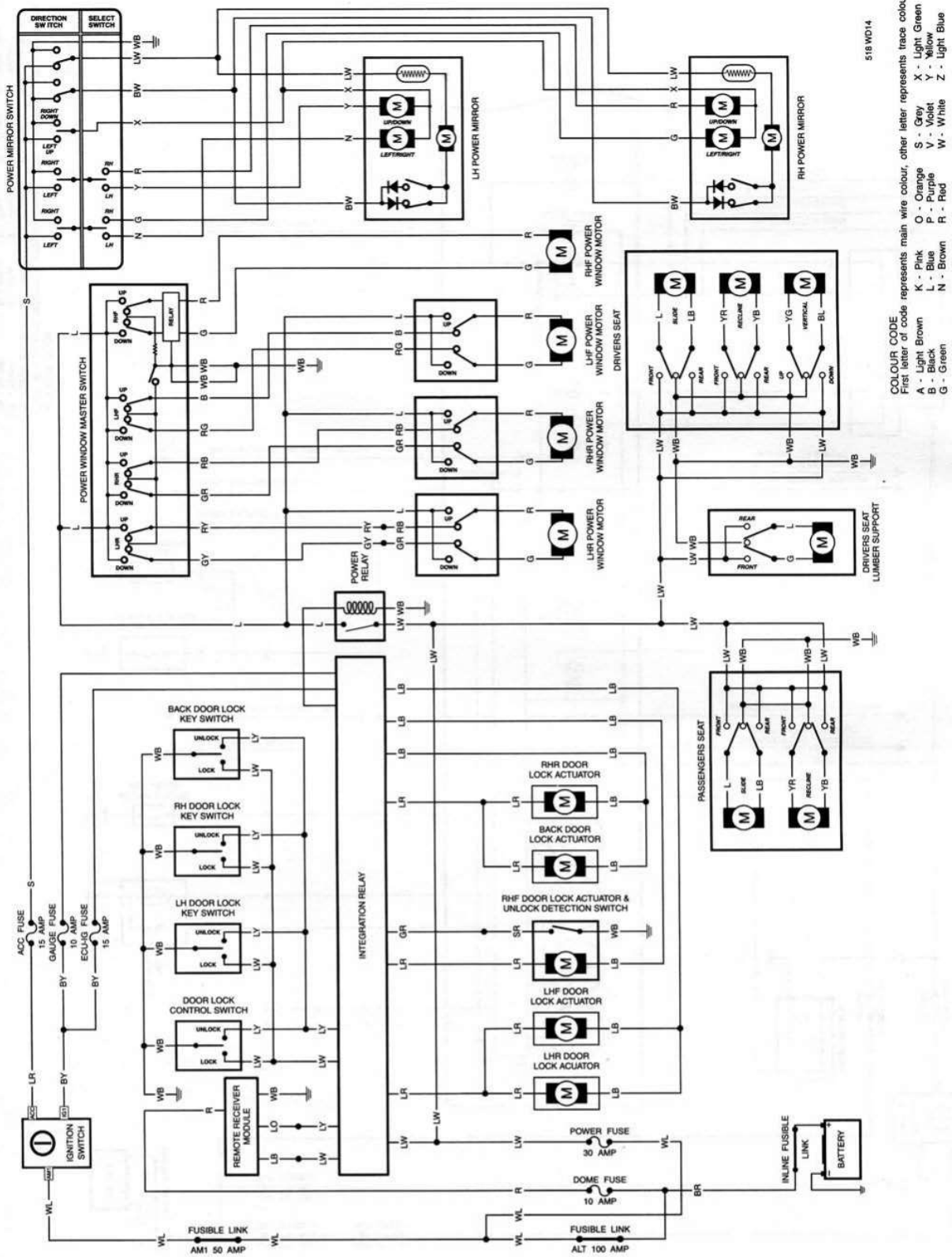
Power door locks, power windows, power mirrors and power seats. Late models.
