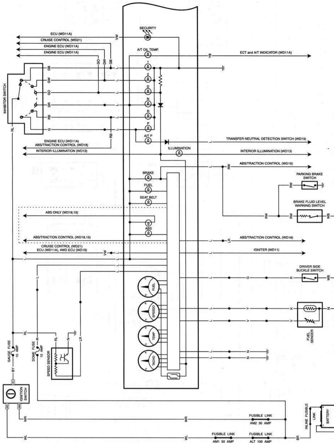
Instrument cluster. Late models.
