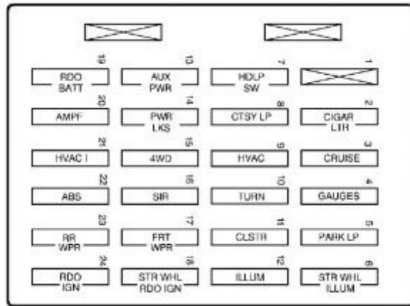
GMC Sonoma mk2 – fuse box – instrument panel
