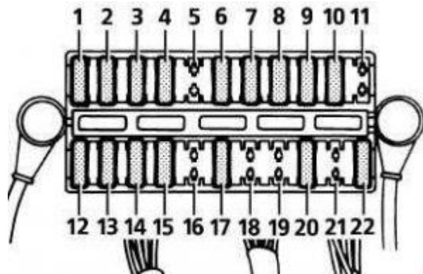
diagram – right hand seat fuse box
