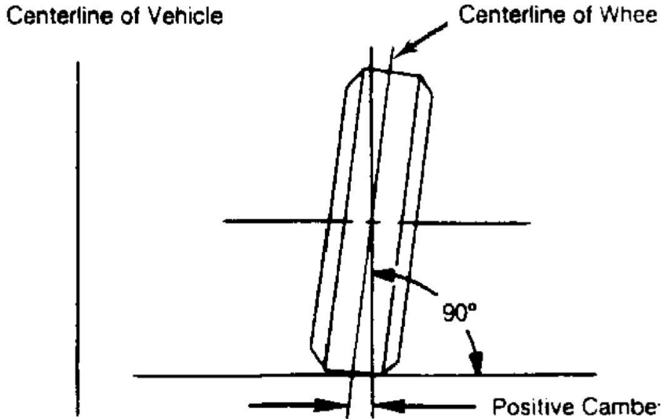
Fig. 3: Determining Camber Angle
