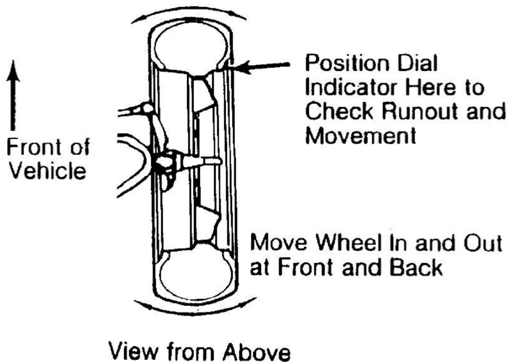
Fig. 1: Checking Steering Linkage
