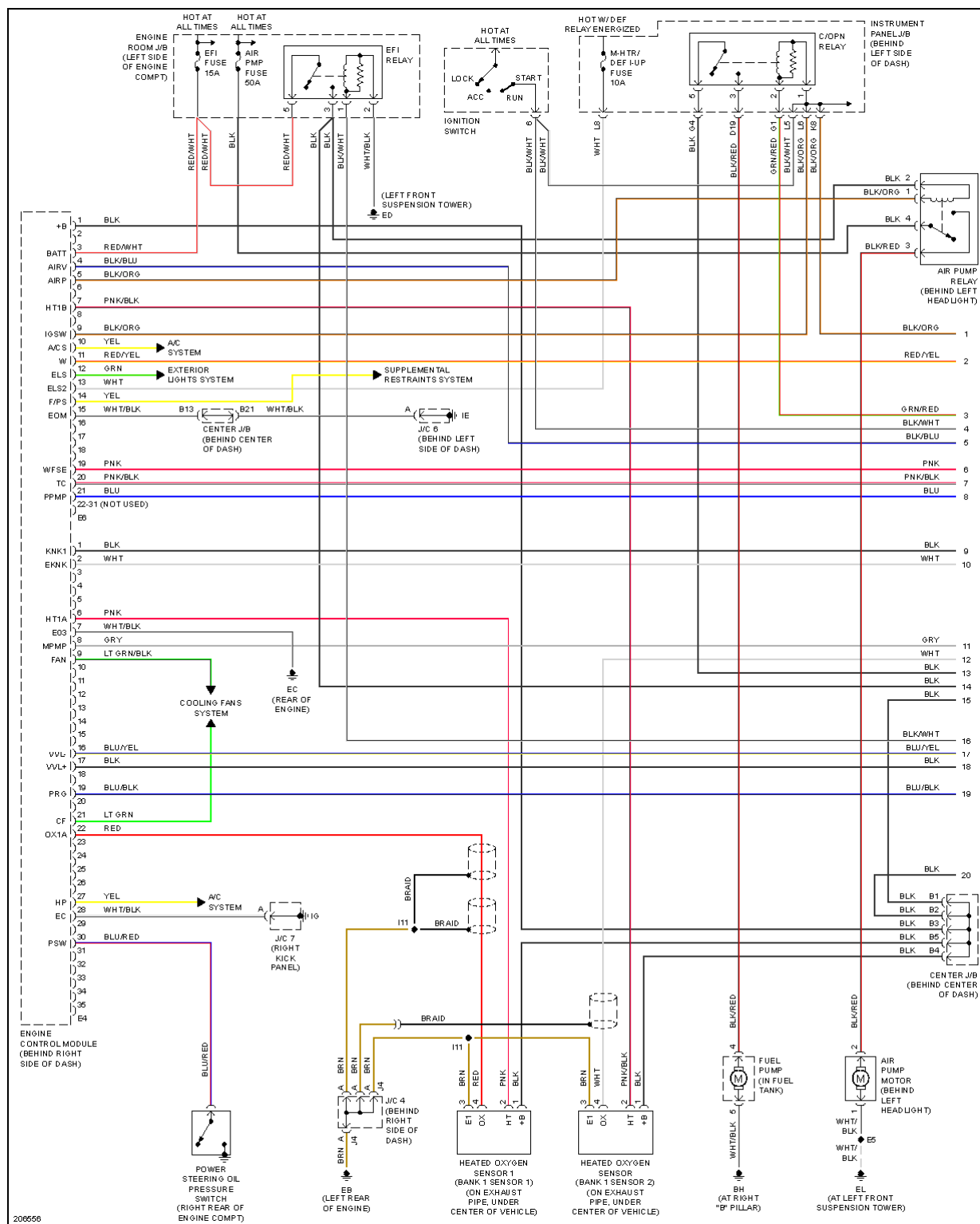
Fig. 18: 1.8L, Engine Performance Circuit, XRS (1 of 3)
