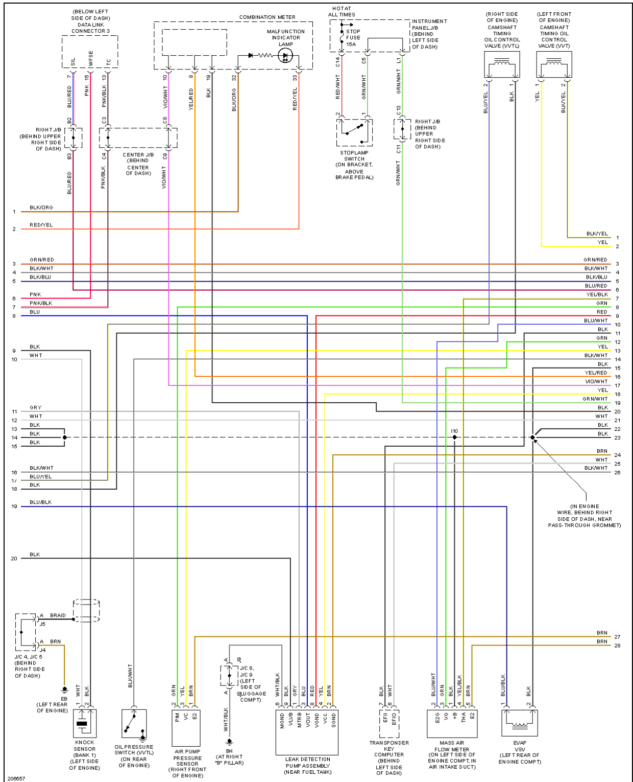
Fig. 19: 1.8L, Engine Performance Circuit, XRS (2 of 3)
