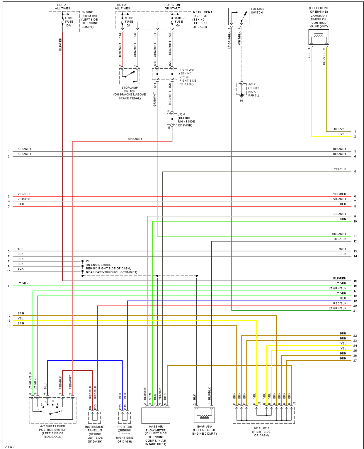
Fig. 16: 1.8L, Engine Performance Circuit, Except XRS (3 of 4)
