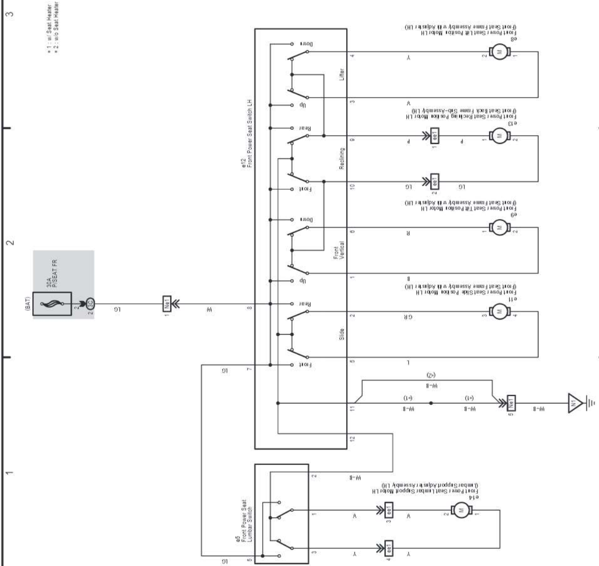
Power Seat (Driver' s Seat) (TMMK Made)
